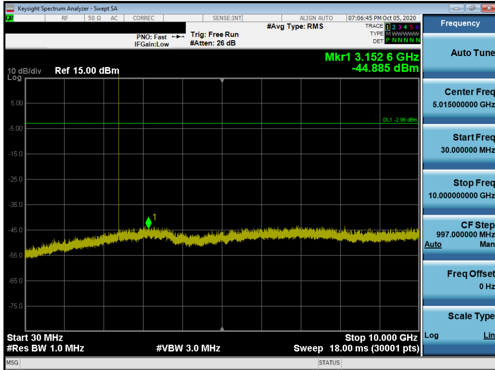
Plot 7-107. Conducted Spurious Plot (Bluetooth, 1#REF!Mbps – Ch. 0)
