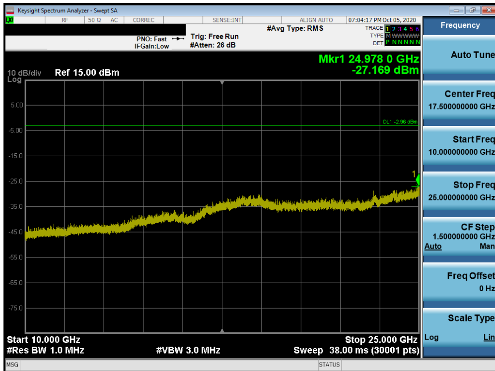
Plot 7-108. Conducted Spurious Plot (Bluetooth, 1#REF!Mbps – Ch. 0)
