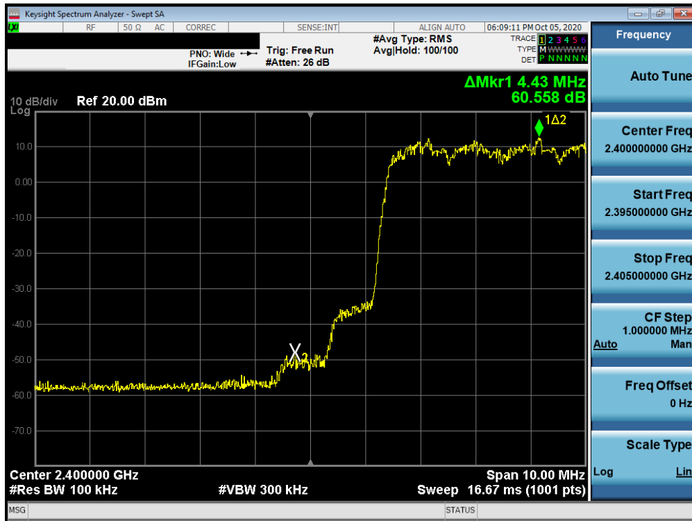
Plot 7-93. Band Edge Plot (Bluetooth with Hopping Enabled, ANT1 - 3 Mbps)
