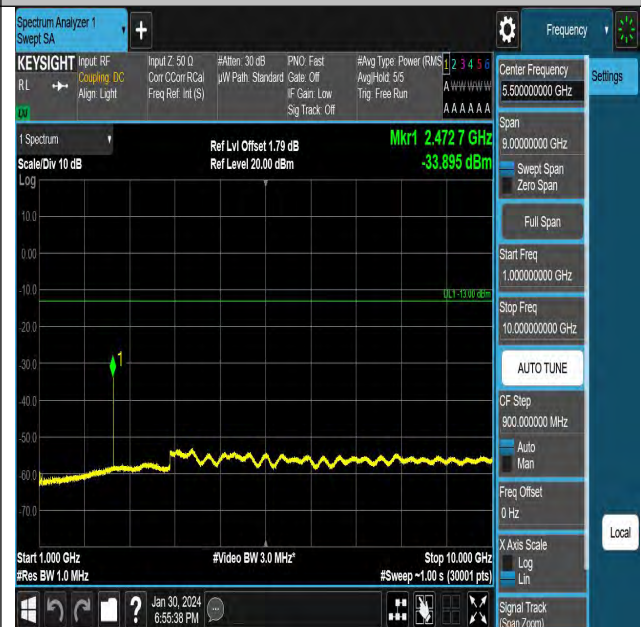
EGPRS850-128-8-1000~10000MHz-PASS
