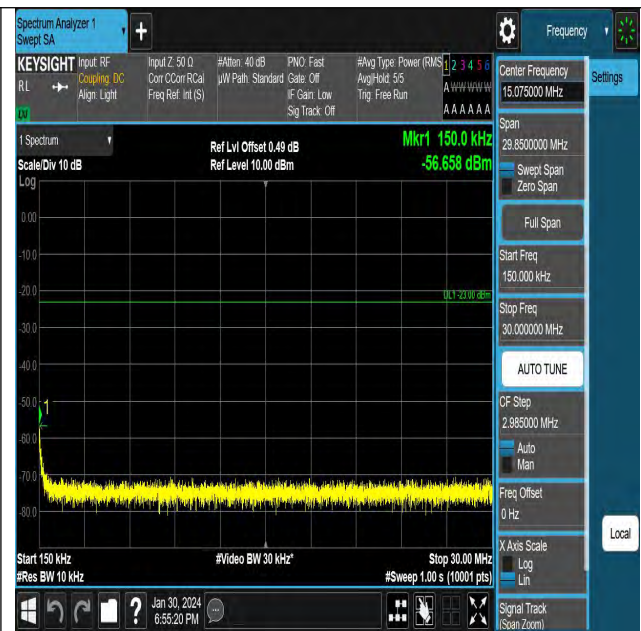
EGPRS850-128-8-0.15~30MHz-PASS
