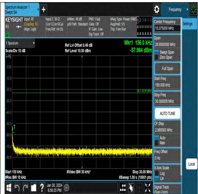
EGPRS850-251-8-0.15~30MHz-PASS
