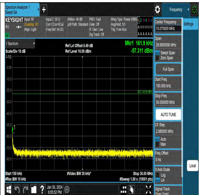
EGPRS850-190-8-0.15~30MHz-PASS
