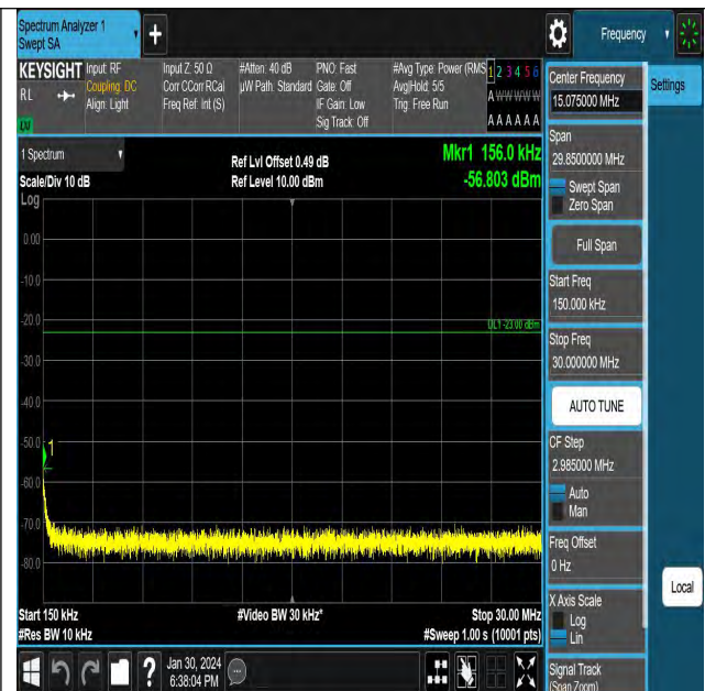
GPRS850-190-5-0.15~30MHz-PASS
