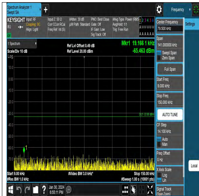
EGPRS850-128-8-0.009~0.15MHz-PASS
