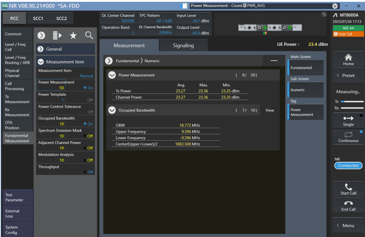
Call box 5G NR setup screenshot
