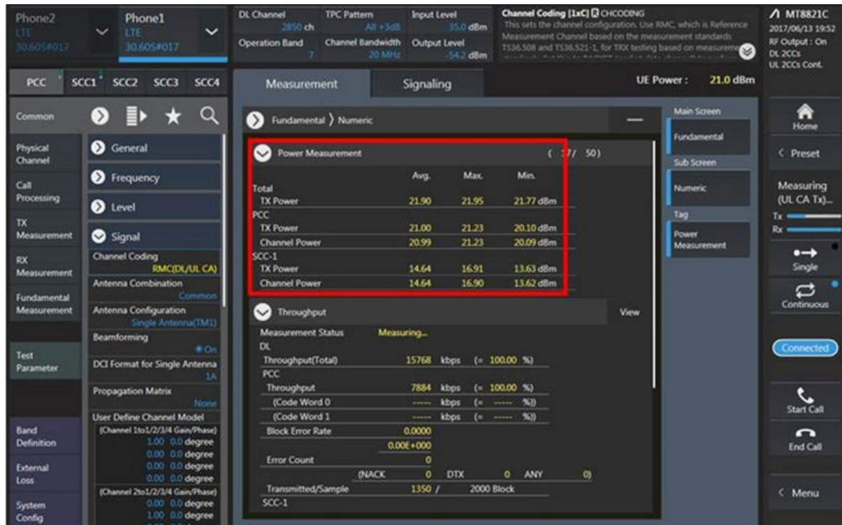
Call box ULCA setup screenshot
