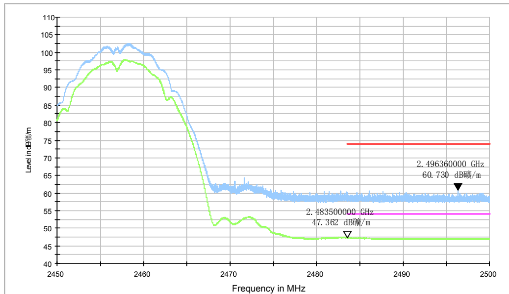
Fig.A.6.2.4 Transmitter Spurious Emission - Radiated (Power): 802.11b, ch10, 2.45 GHz - 2.50GHz
