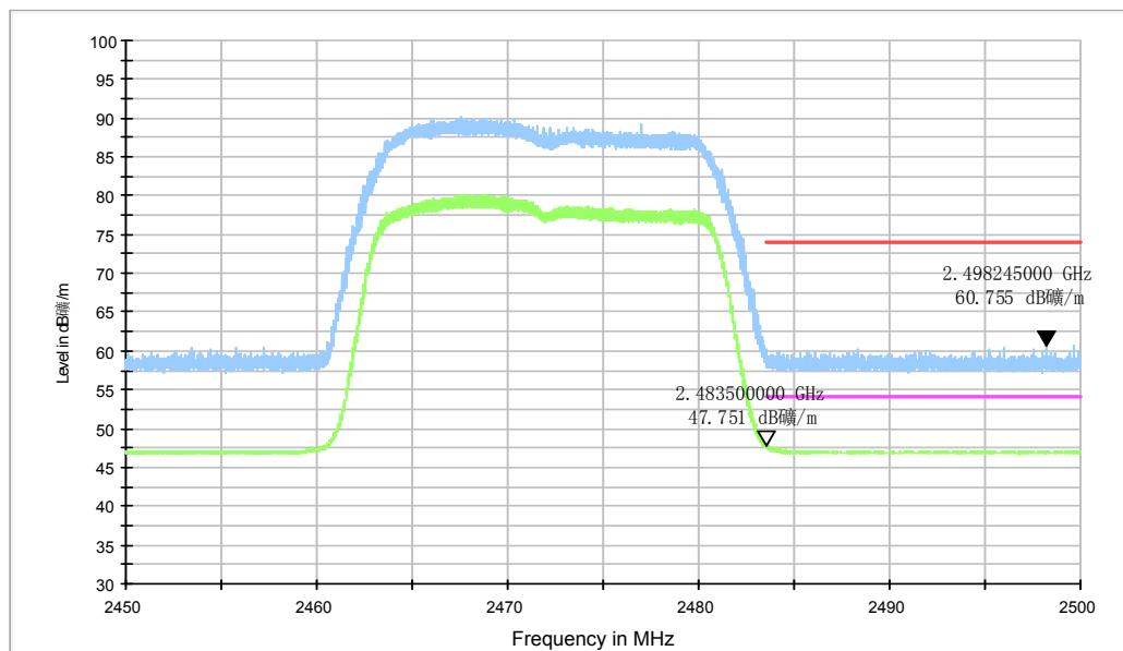
Fig.A.6.2.18 Transmitter Spurious Emission - Radiated (Power): 802.11n-HT20, ch13, 2.45 GHz - 2.50GHz
