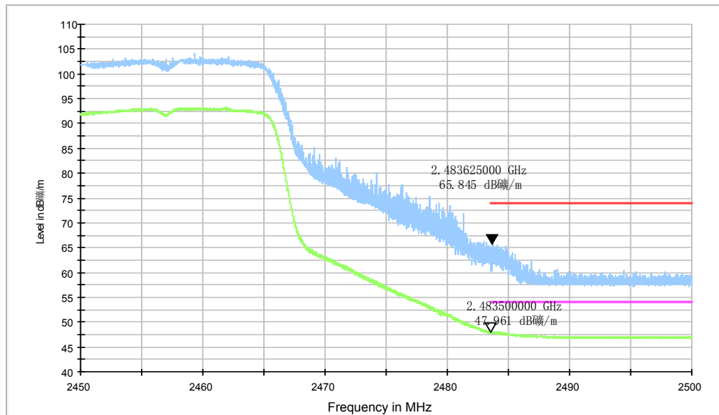
Fig.A.6.2.16 Transmitter Spurious Emission - Radiated (Power): 802.11n-HT20, ch10, 2.45 GHz - 2.50GHz
