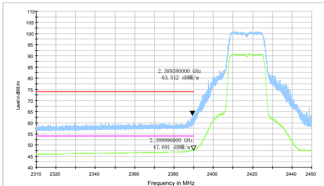
Fig.A.6.2.15 Transmitter Spurious Emission - Radiated (Power): 802.11n-HT20, ch2, 2.31 GHz - 2.45GHz
