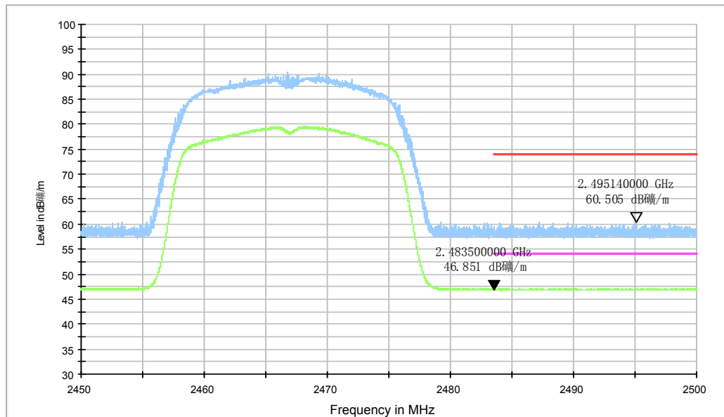
Fig.A.6.2.17 Transmitter Spurious Emission - Radiated (Power): 802.11n-HT20, ch12, 2.45 GHz - 2.50GHz
