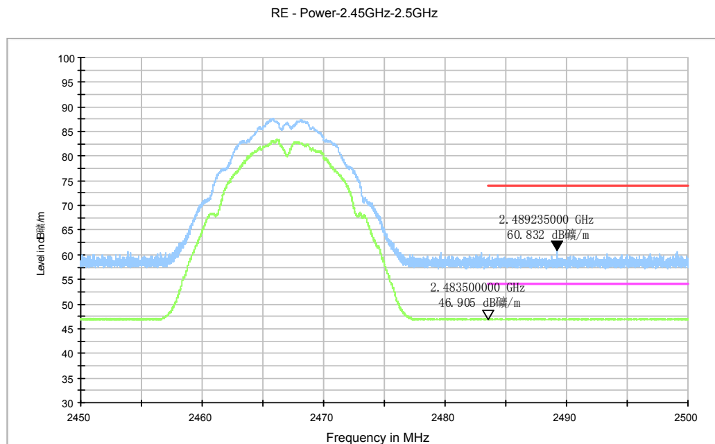
Fig.A.6.2.5 Transmitter Spurious Emission - Radiated (Power): 802.11b, ch12, 2.45 GHz - 2.50GHz
