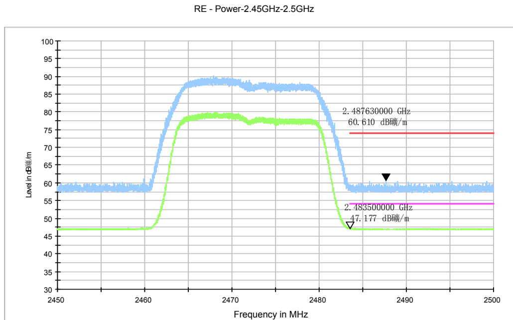
Fig.A.6.2.11 Transmitter Spurious Emission - Radiated (Power): 802.11g, ch12, 2.45 GHz - 2.50GHz
