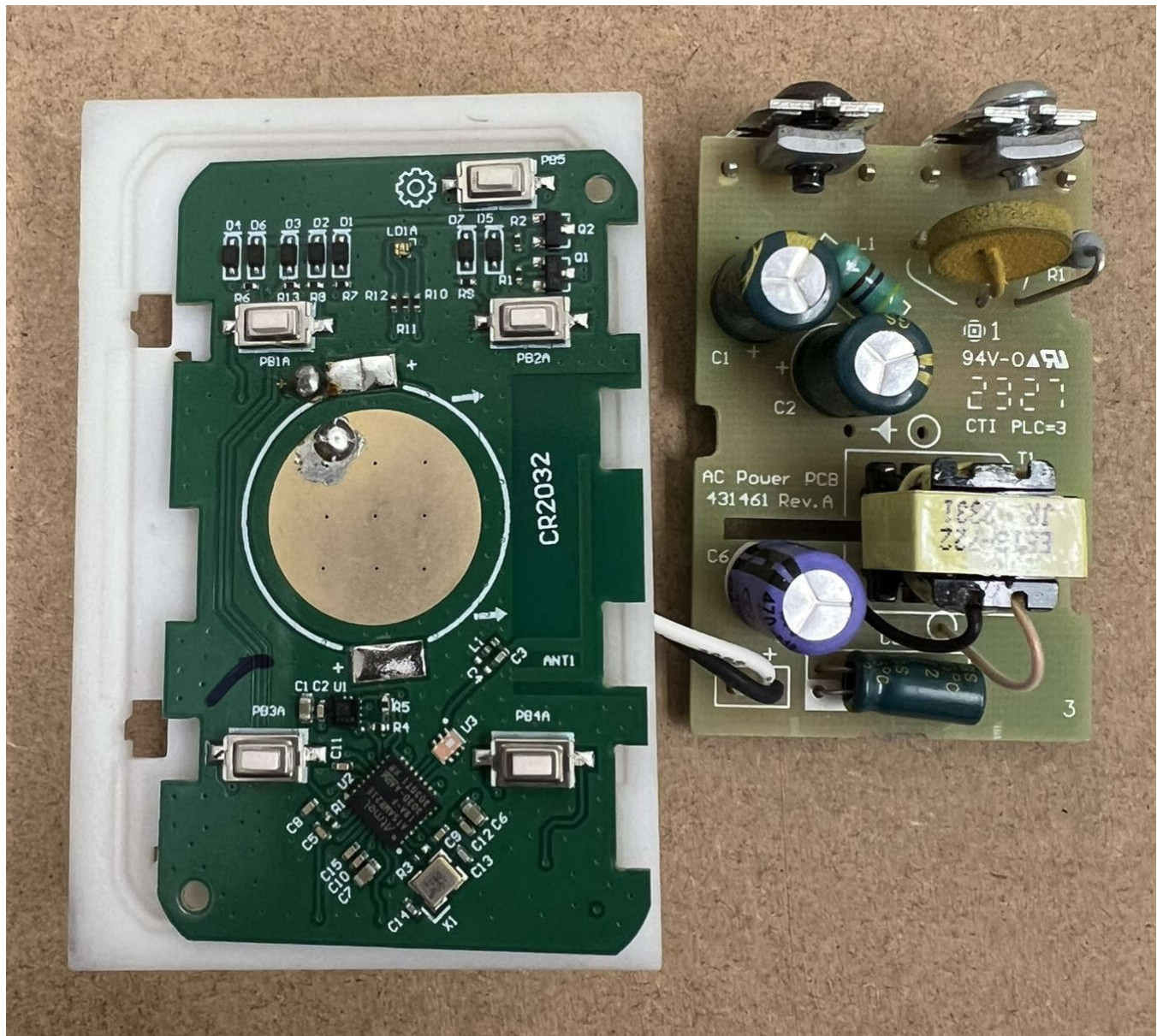
WNACB46 RF Board -Top (Left), AC Board Bottom (Right)
