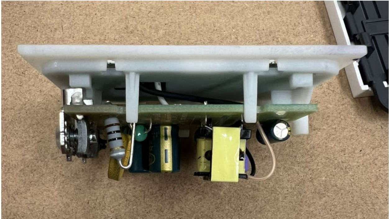
WNACB46 Back Cover Removed
