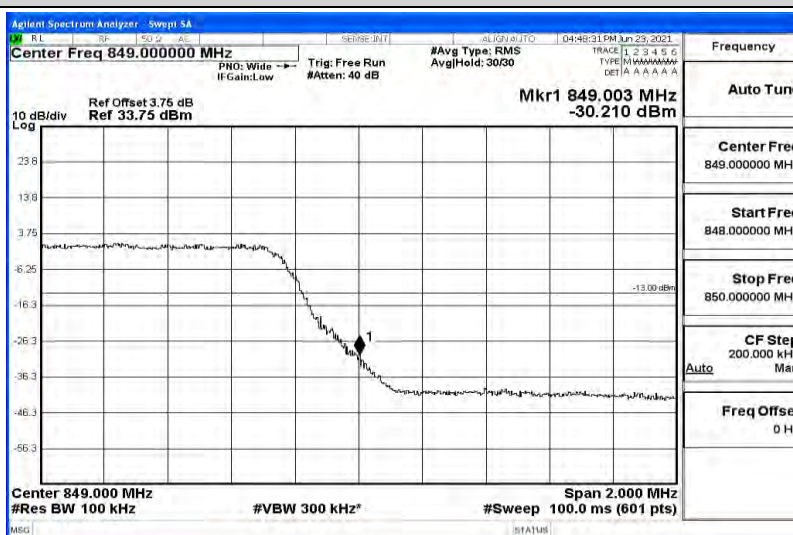
Band5-5MHz-16QAM-20425-25RB#0
