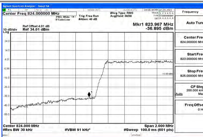
Band5-1.4MHz-16QAM-20643-6RB#0
