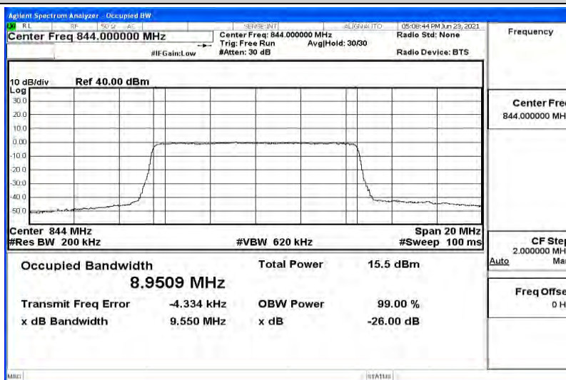
Band5-10MHz-16QAM-20600-50RB#0-8.9509
