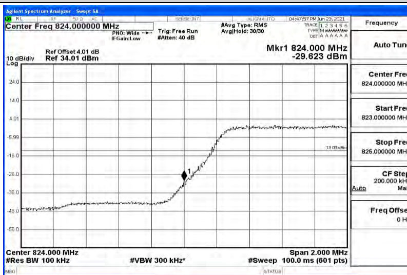
Band5-5MHz-QPSK-20625-25RB#0
