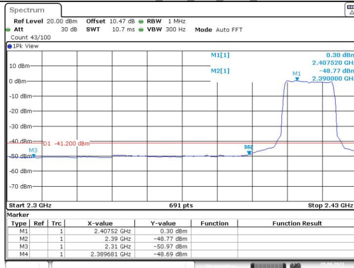
11N20SISO Ant1 Low 2412 Peak
