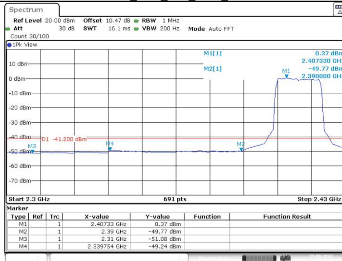
11G Ant1 Low 2412 Peak
