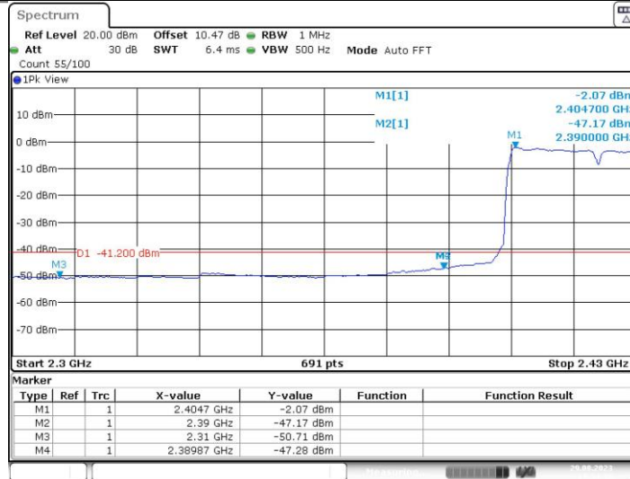
11N40SISO Ant1 Low 2422 Peak
