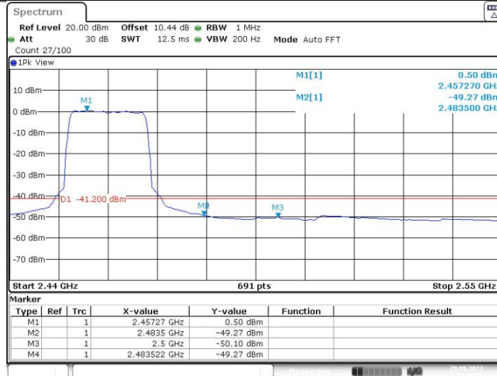
11G Ant1 High 2462 Peak
