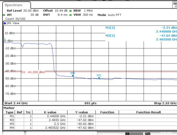
11N40SISO Ant1 High 2452 Peak
