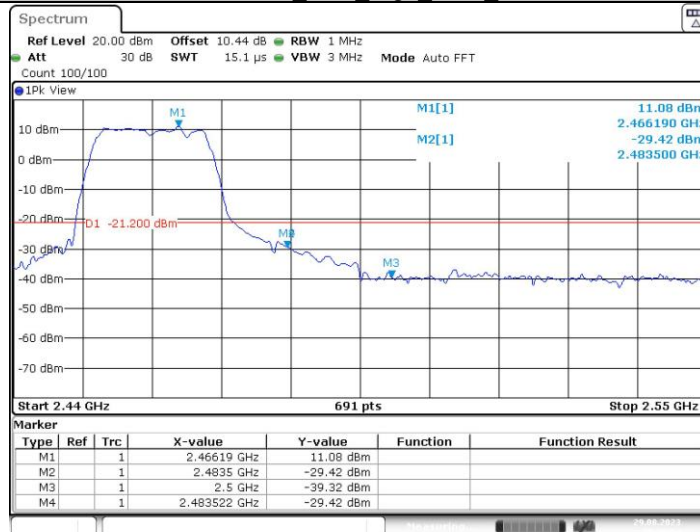
11N20SISO Ant1 High 2462 Peak
