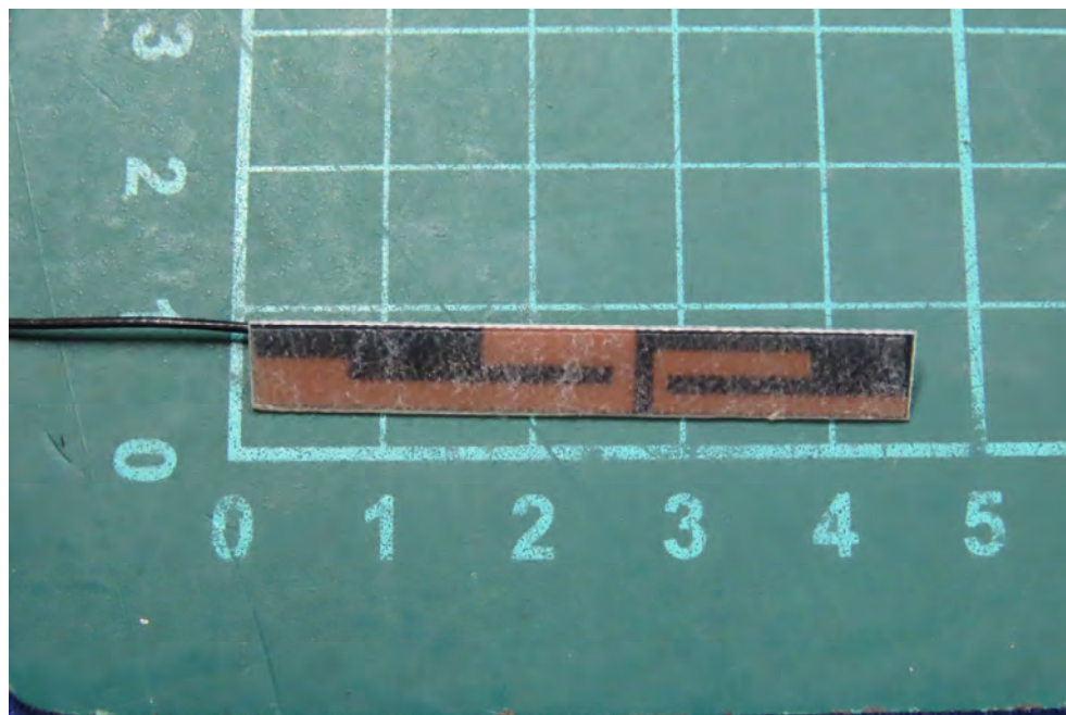
(34) EUT Photo
