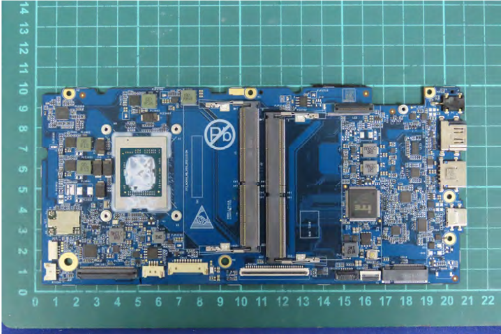
(22) EUT Photo
