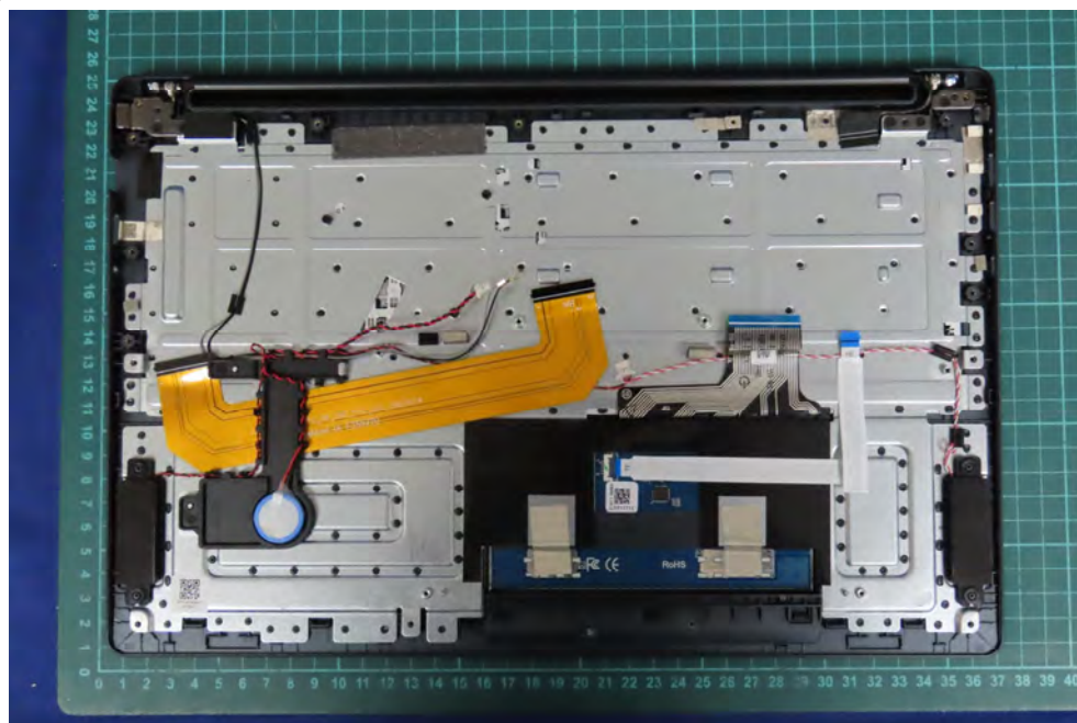
(27) EUT Photo
