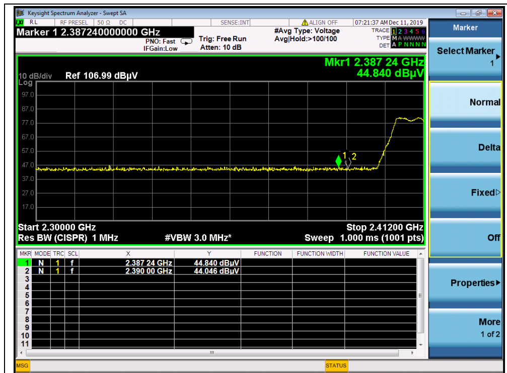
(AVG, Channel 1, 802.11g)
