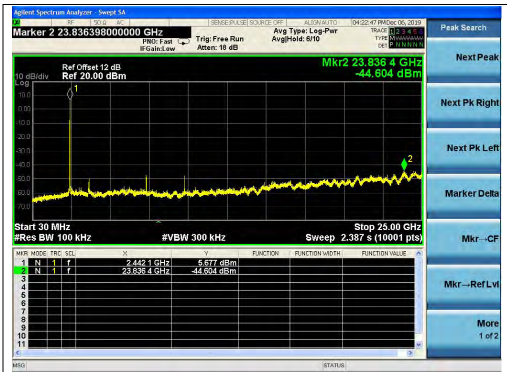
(Channel 7, 30MHz to 25GHz)
