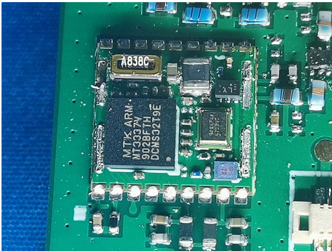
GPS Chip
