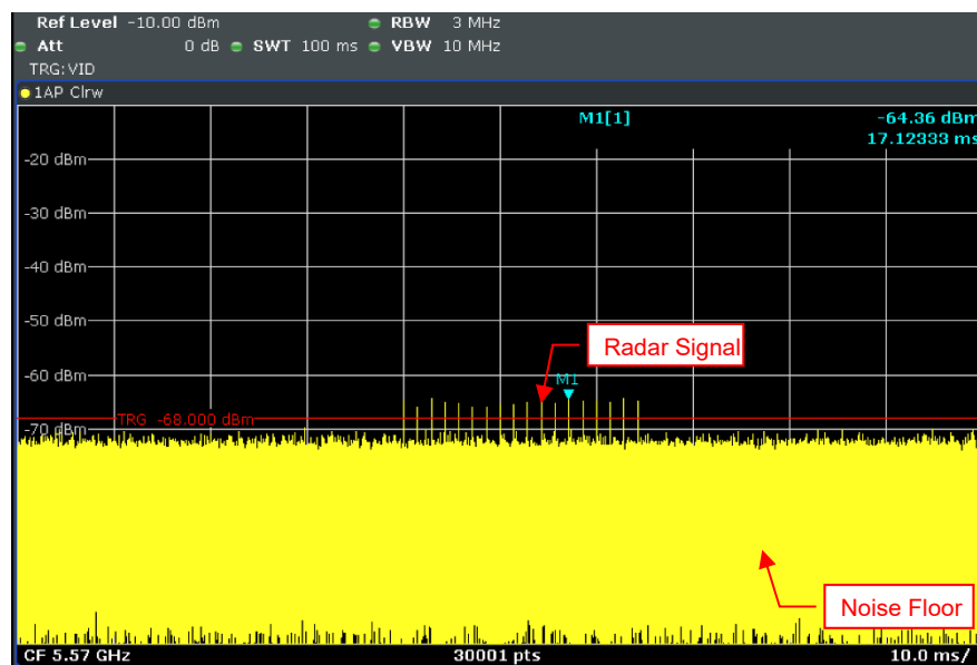
Radar Signal 0
