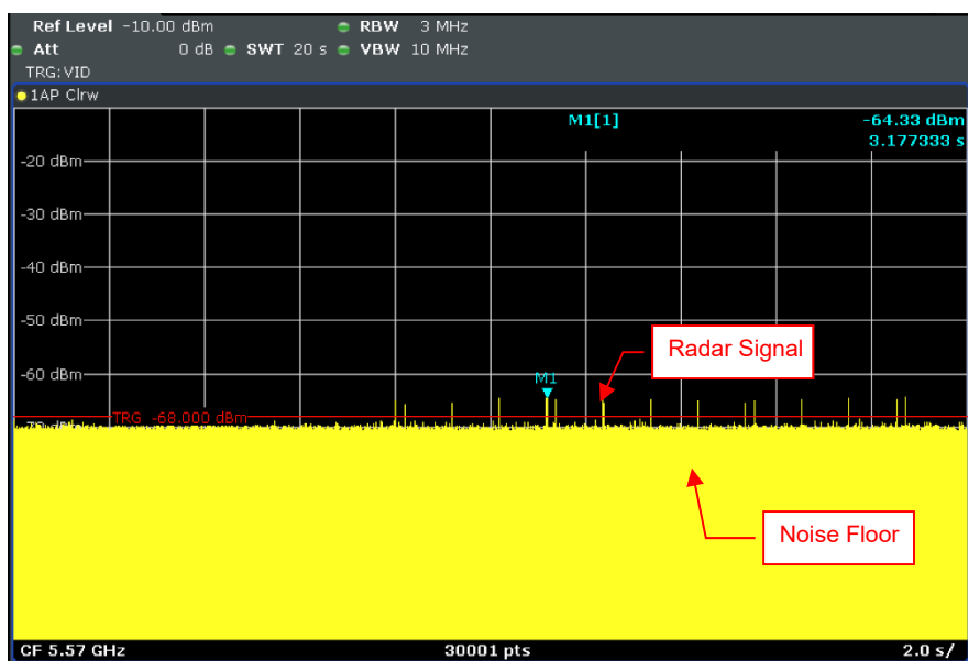
Radar Signal 5
