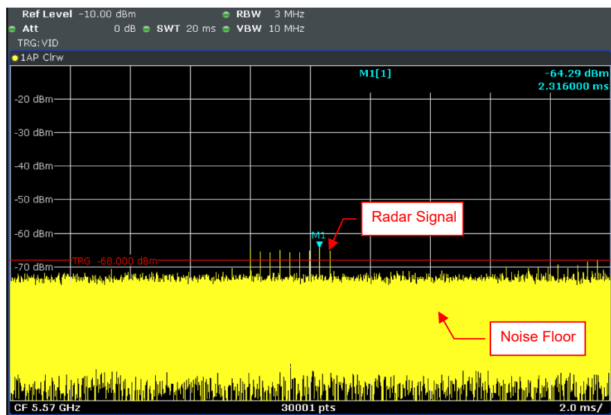
Radar Signal 6
