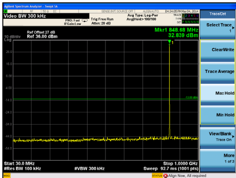
(Plot A3:GSM 850MHz Channel = 251, 30MHz to 1GHz)
