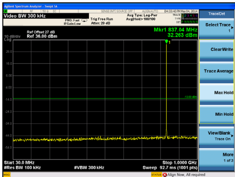
(Plot A2:GSM 850MHz Channel = 190, 30MHz to 1GHz)
