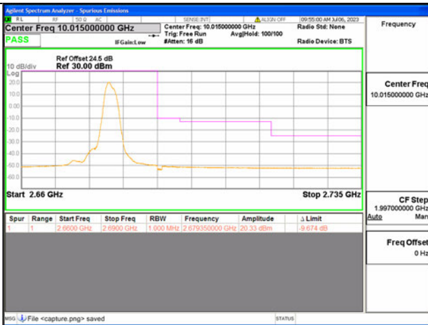
41C / 15+10MHz / High CH / QPSK / 1#74-1#0
