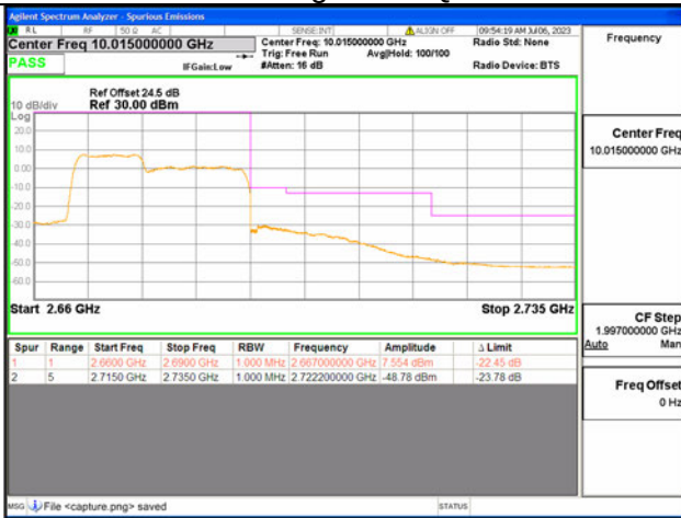
41C / 10+15MHz / High CH / QPSK / 50#0-75#0
