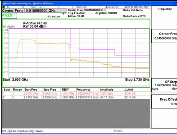
41C / 10+20MHz / High CH / QPSK / 50#0-100#0
