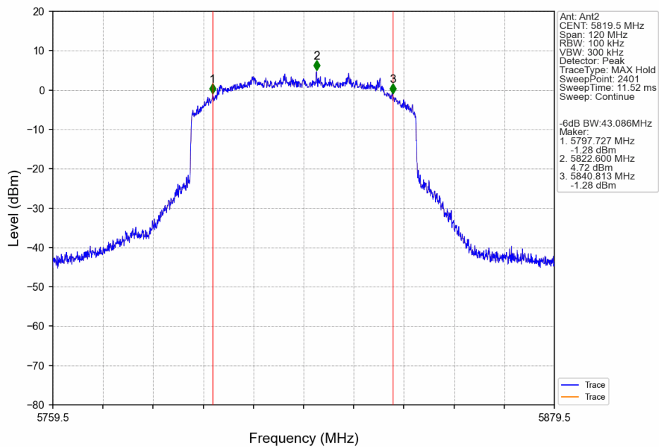
60M_HCH_5819.5MHz_Ant2-NTNV
