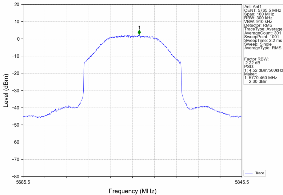
80M_LCH_5765.5MHz_Ant1_NTNV
