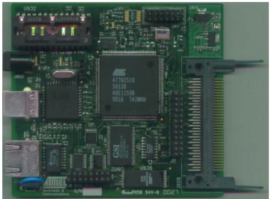
Figure 2-1. AP development board
