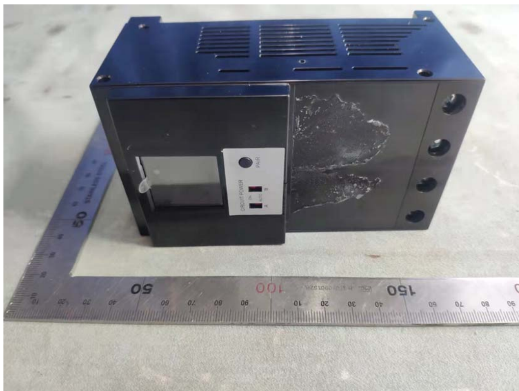
FIGURE 2 QO 60A RELAYWITH CURENT TRANSFORMER PON (M/N: GPM-QP1R60240-21) BACK
