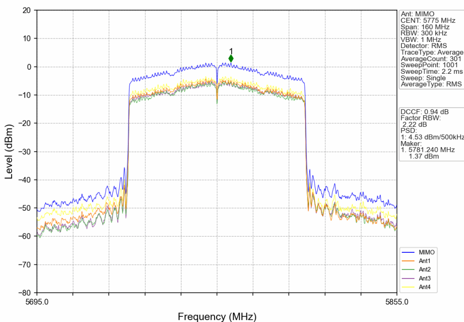
802.11ax(HEW80)_MCH_5775MHz_RU996_Left_MIMO_NTNV
