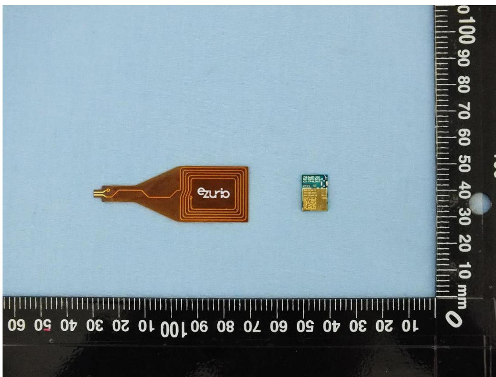
Integrated Antenna
