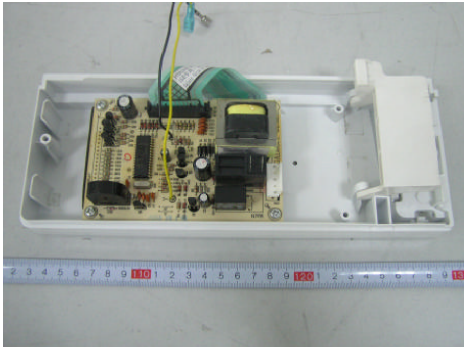
EUT-Controller panel view(1)
