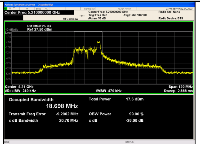
IEEE 802.11ax_Channel 42_80MHz_Antenna 1_RU&amp;Index 26RU17
