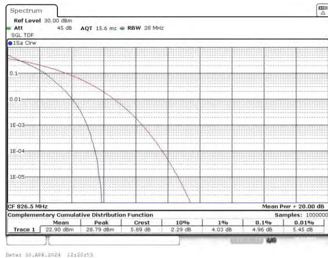
Band5-5MHz-QPSK-20525-25RB#0
