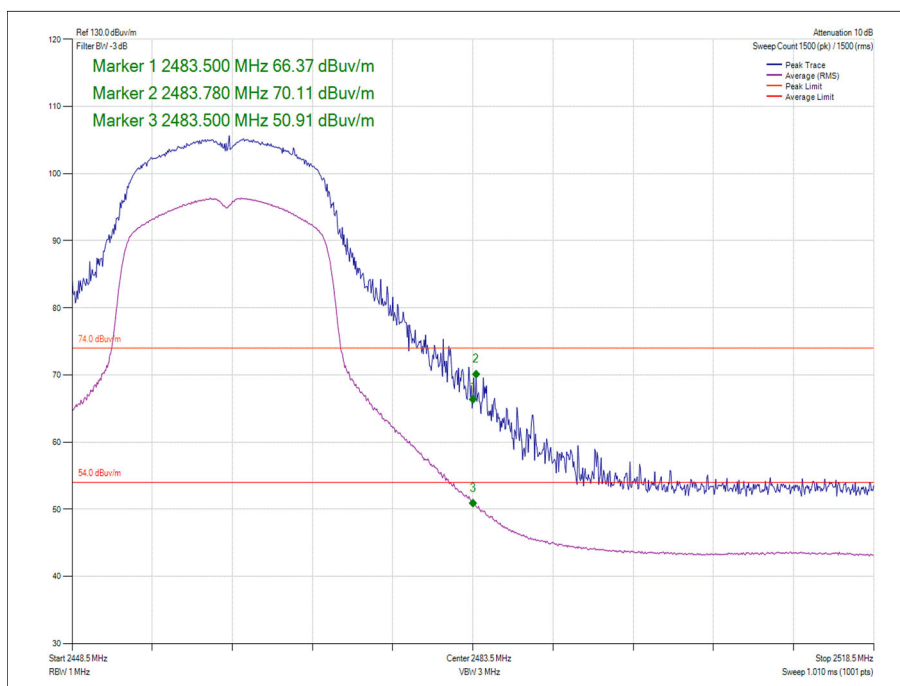
Figure 30 - Data Rate/MCS with the Highest Power - MCS0 2462 MHz - Band Edge Frequency 2483.5 MHz
