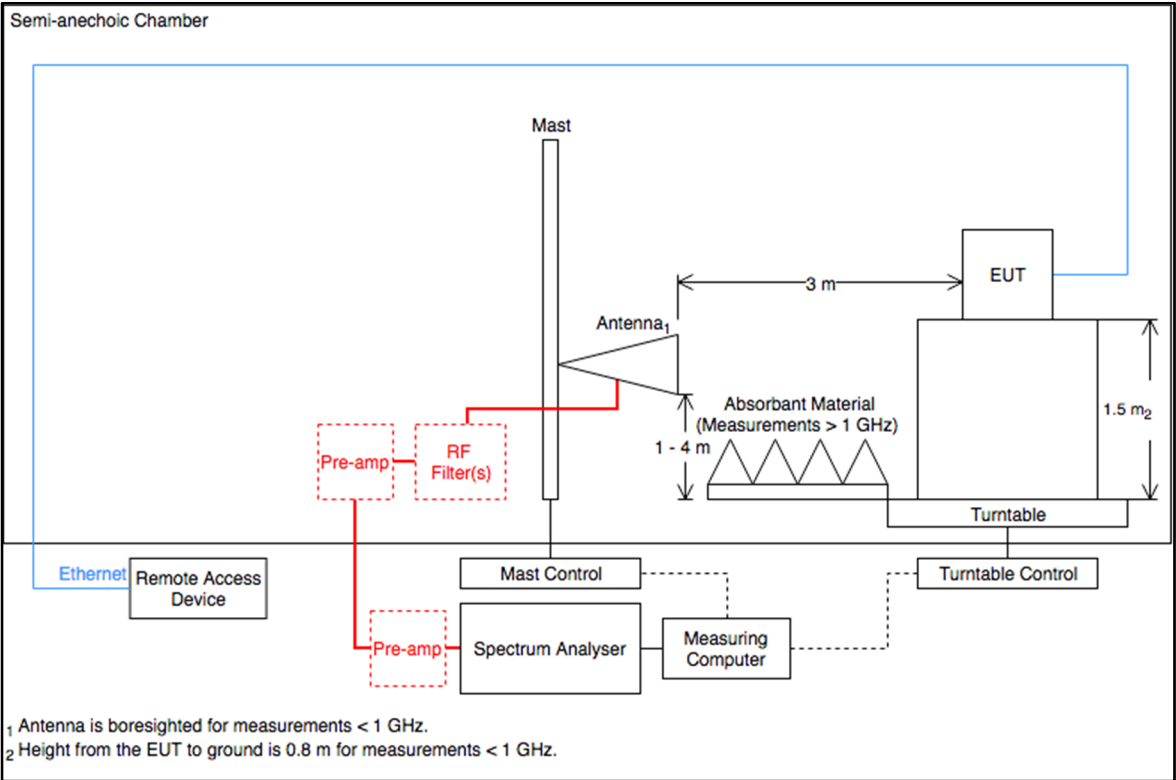
Figure 37 - Setup Diagram
