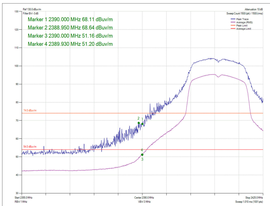
Figure 25 - Data Rate/MCS with the Highest Power - 6 Mbps 2412 MHz - Band Edge Frequency 2390 MHz
