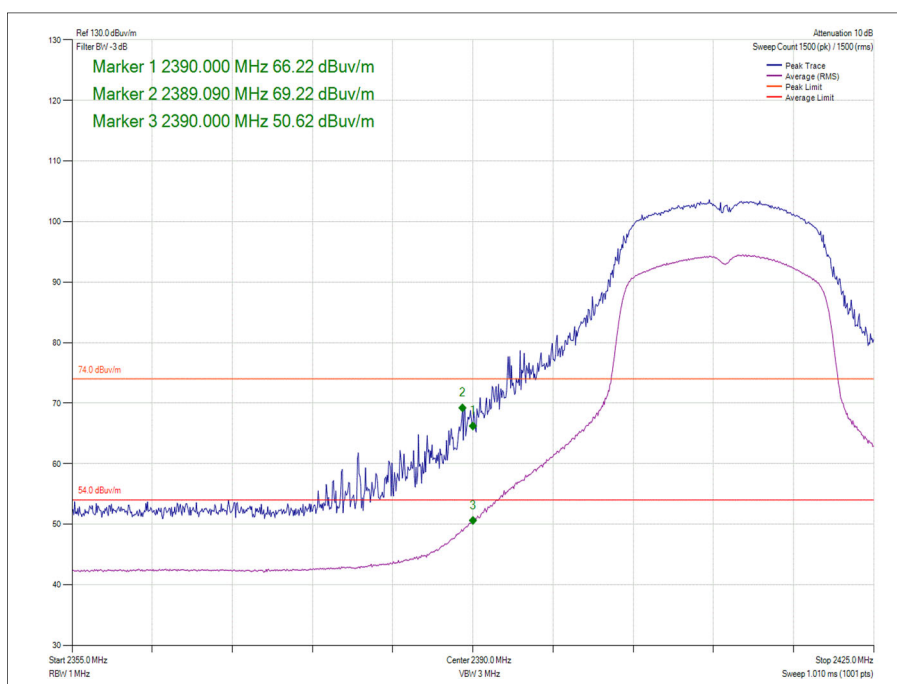
Figure 29 - Data Rate/MCS with the Highest Power - MCS0 2412 MHz - Band Edge Frequency 2390 MHz
