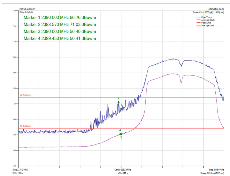
Figure 33 - Data Rate/MCS with the Highest Power - MCS0 2422 MHz - Band Edge Frequency 2390 MHz
