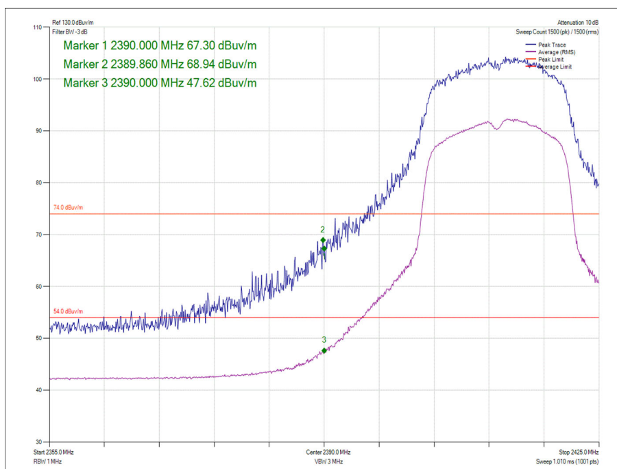
Figure 31 - Data Rate/MCS with the Widest Bandwidth - MCS6 2412 MHz - Band Edge Frequency 2390 MHz
