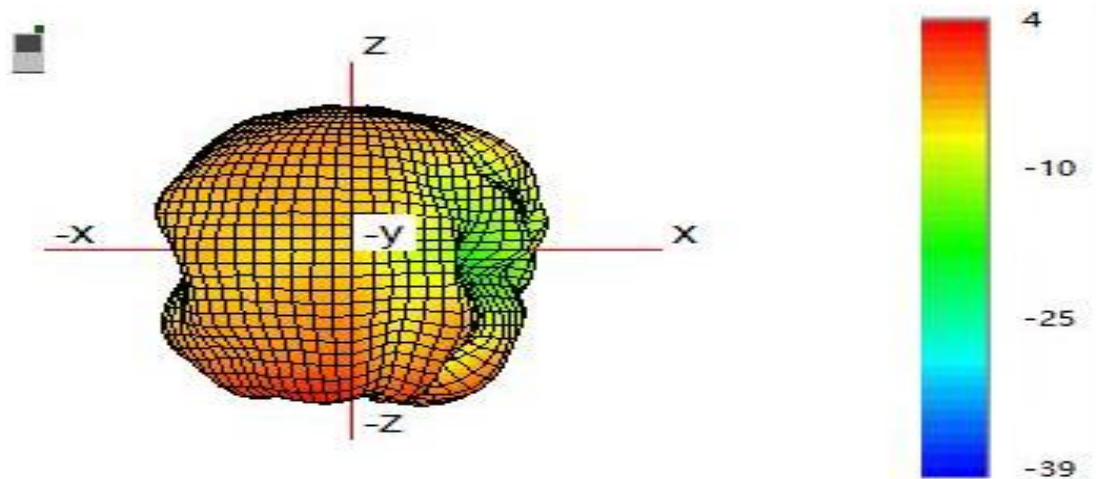
(5)Typical Free Space 3D Radiation Pattern at 5.9GHz(unit:dBi):
