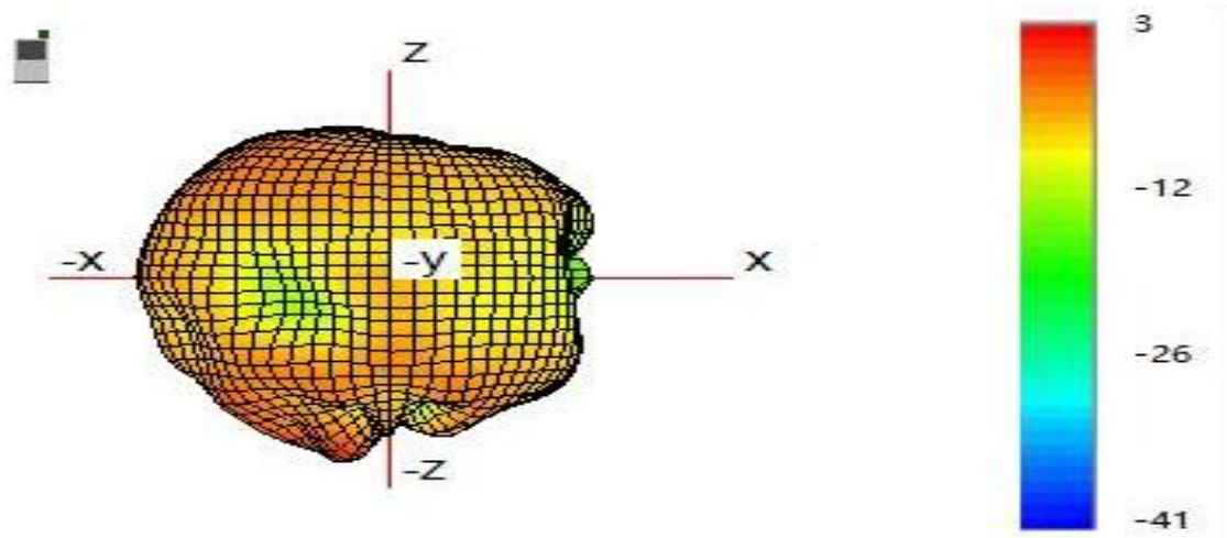
(5)Typical Free Space 3D Radiation Pattern at 5.9GHz(unit:dBi):
