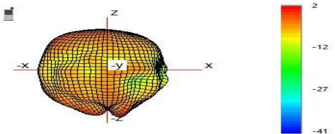
(5)Typical Free Space 3D Radiation Pattern at 6GHz(unit:dBi):
