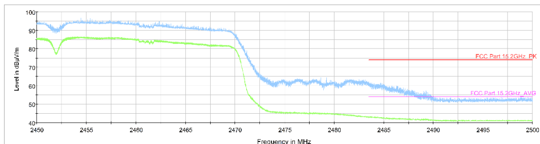
Fig.A.6.2.8 Transmitter Spurious Emission - Radiated (Power): 802.11n-HT40, ch9, 2.45 GHz - 2.50GHz
