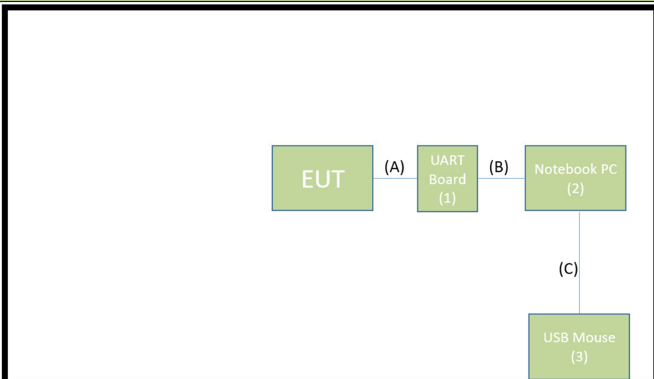
Connection Diagram
