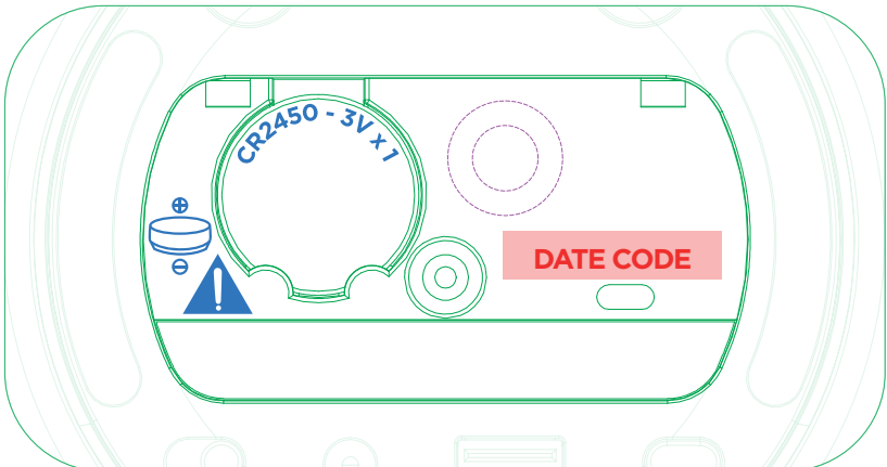
BATTERY DOOR INTERIOR GAW
