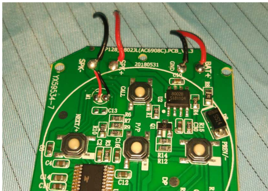
EUT – IC View 1
