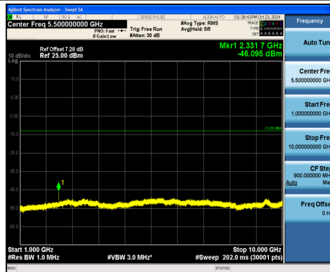
Band13-5MHz-QPSK-23205-1-0-Low-1000-10000--46.1-PASS
