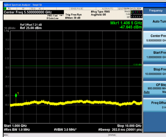
Band12-10MHz-QPSK-23095-1-0-Low-1000-10000--47.65-PASS
