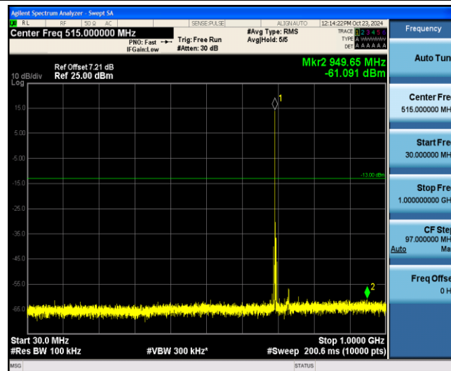
Band12-10MHz-16QAM-23060-1-0-Low-30-1000--61.09-PASS
