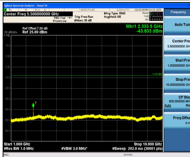
Band13-10MHz-QPSK-23230-1-0-Low-1000-10000--43.83-PASS
