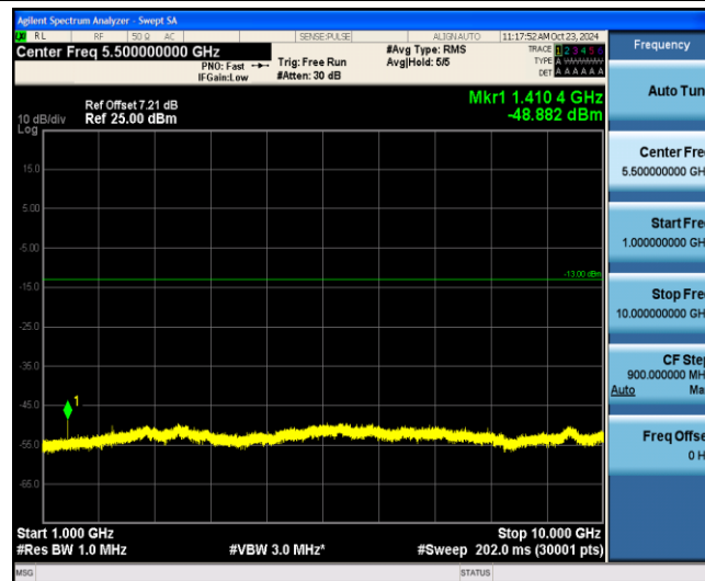
Band12-5MHz-16QAM-23095-1-0-Low-1000-10000--48.88-PASS
