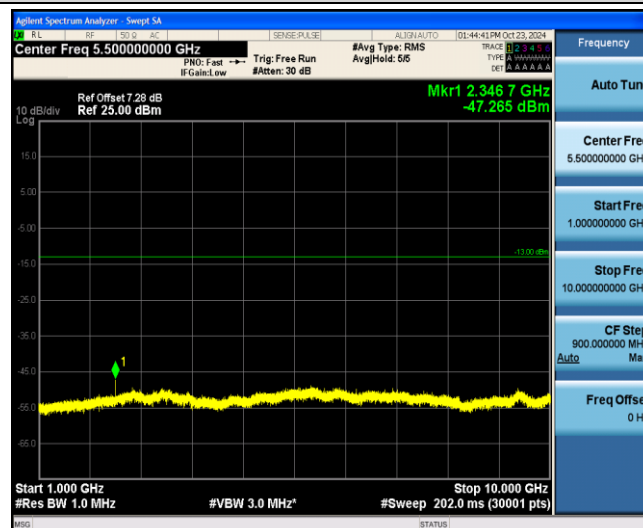
Band13-5MHz-16QAM-23255-1-0-Low-1000-10000--47.27-PASS
