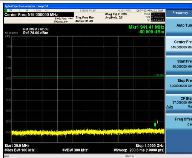
Band2-1.4MHz-16QAM-18607-1-0-Low-30-1000--60.51-PASS
