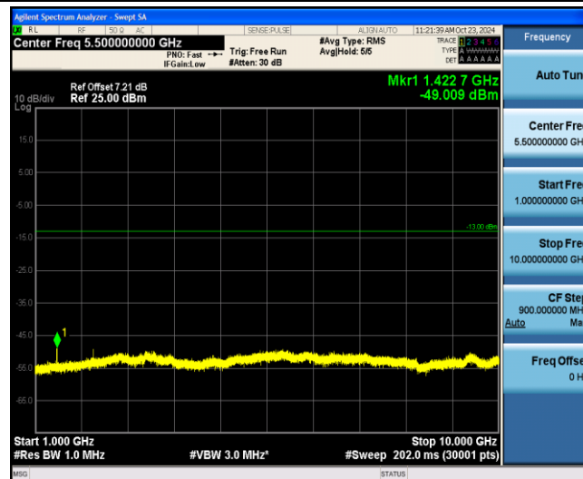
Band12-5MHz-16QAM-23155-1-0-Low-1000-10000--49.01-PASS
