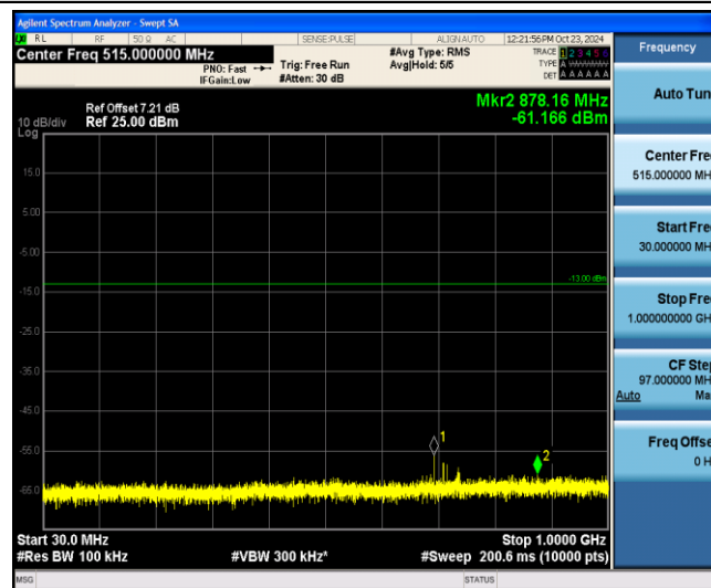
Band12-10MHz-16QAM-23130-1-0-Low-30-1000--61.17-PASS
