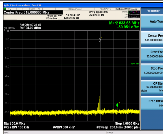
Band12-10MHz-16QAM-23095-1-0-Low-30-1000--59.95-PASS
