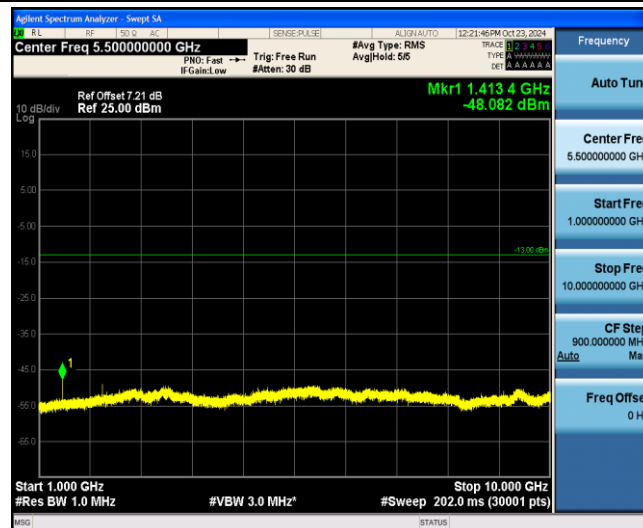
Band12-10MHz-QPSK-23130-1-0-Low-1000-10000--48.08-PASS
