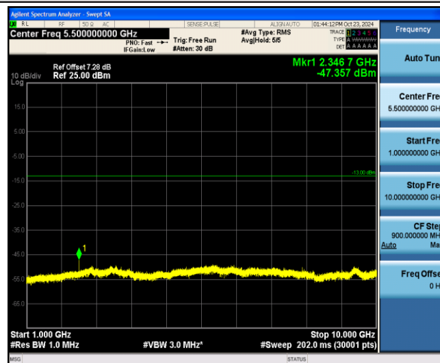
Band13-5MHz-QPSK-23255-1-0-Low-1000-10000--47.36-PASS
