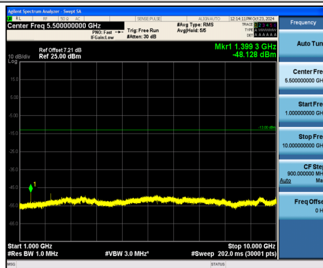
Band12-10MHz-QPSK-23060-1-0-Low-1000-10000--48.13-PASS
