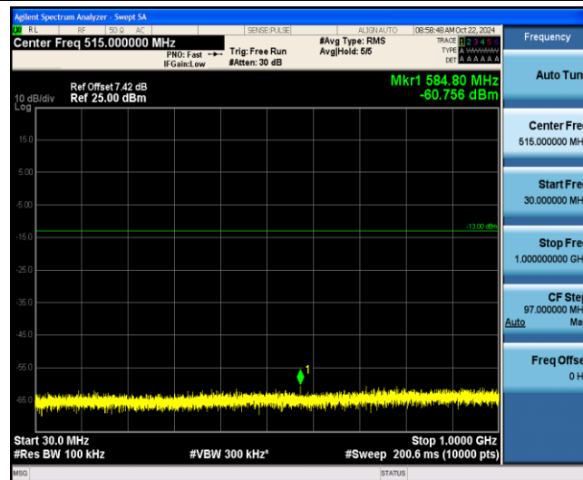
Band2-1.4MHz-QPSK-19193-1-0-Low-30-1000--60.76-PASS
