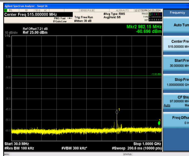
Band12-10MHz-QPSK-23095-1-0-Low-30-1000--60.7-PASS
