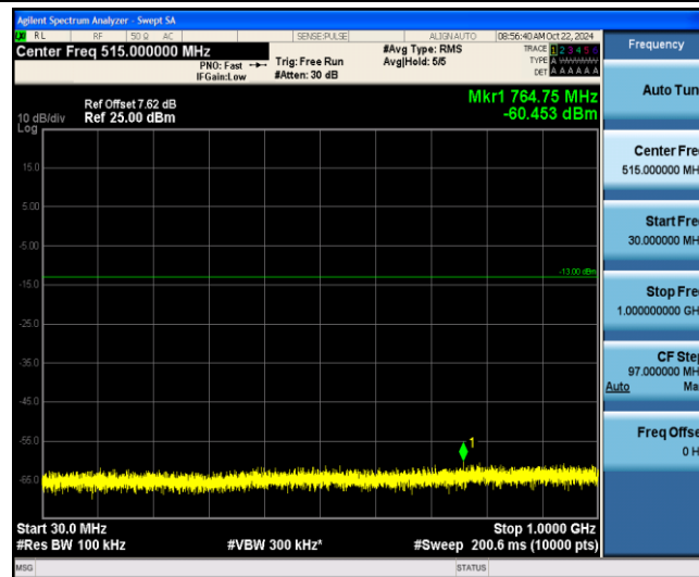
Band2-1.4MHz-QPSK-18607-1-0-Low-30-1000--60.45-PASS
