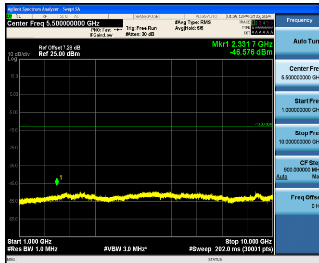
Band13-5MHz-16QAM-23205-1-0-Low-1000-10000--46.58-PASS
