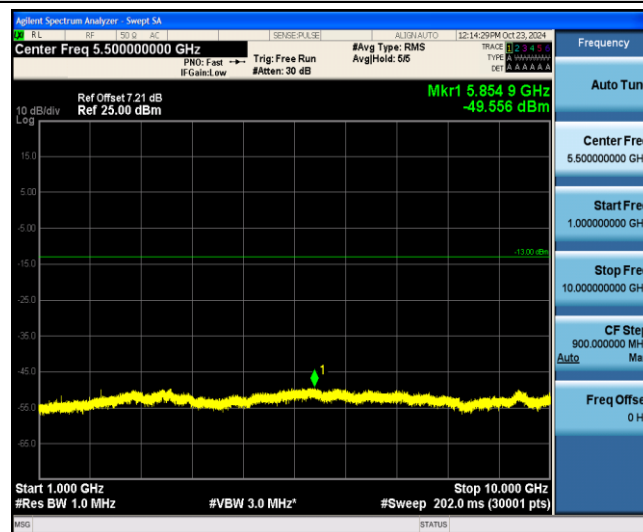
Band12-10MHz-16QAM-23060-1-0-Low-1000-10000--49.56-PASS
