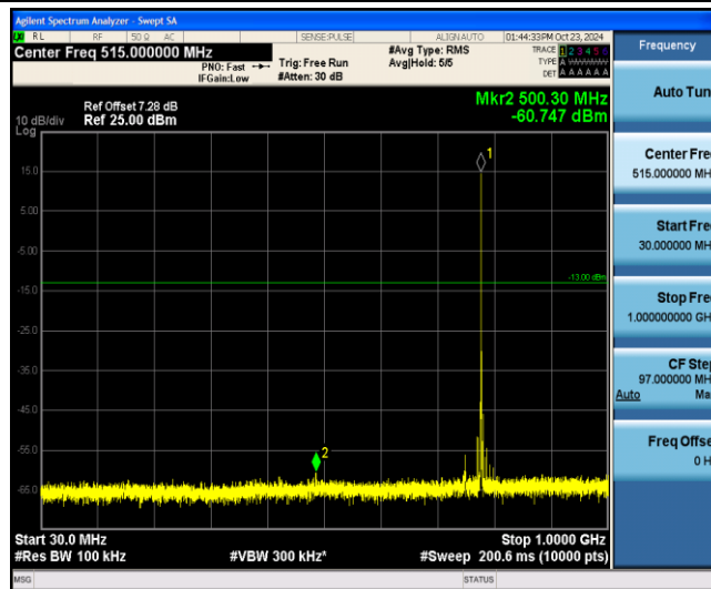
Band13-5MHz-16QAM-23255-1-0-Low-30-1000--60.75-PASS
