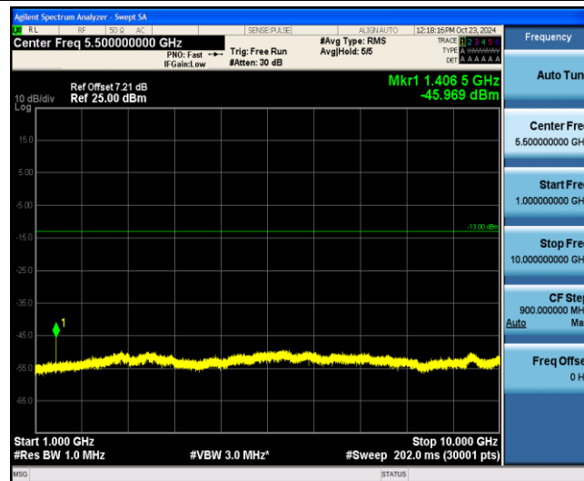
Band12-10MHz-16QAM-23095-1-0-Low-1000-10000--45.97-PASS
