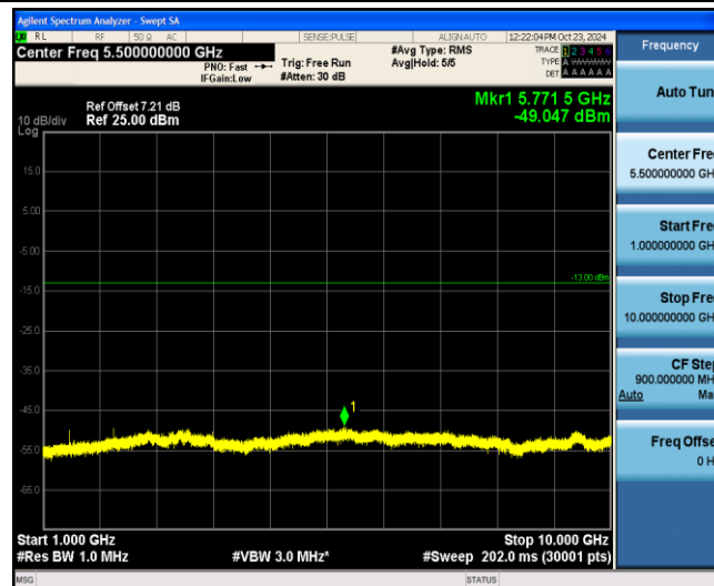
Band12-10MHz-16QAM-23130-1-0-Low-1000-10000--49.05-PASS
