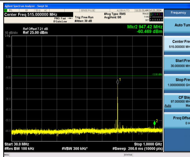
Band12-5MHz-16QAM-23155-1-0-Low-30-1000--60.47-PASS
