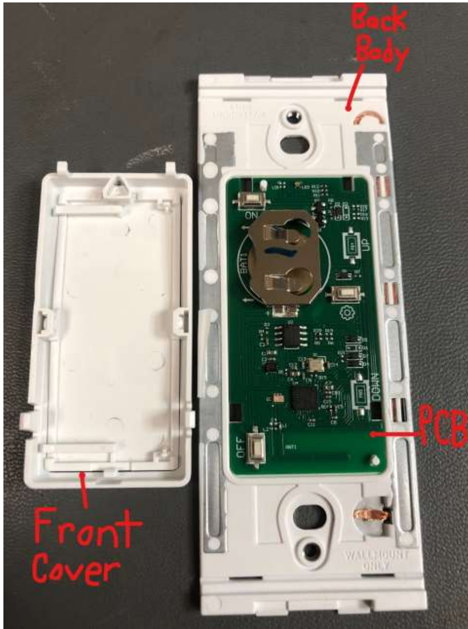
Legrand WNRL43 Switch Assembly View
