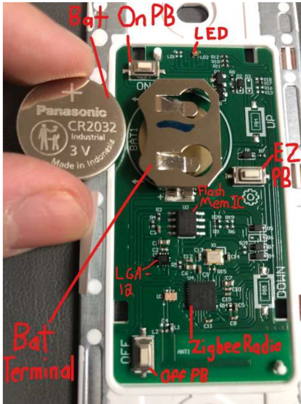
Legrand WNRL43 Switch PCB View
