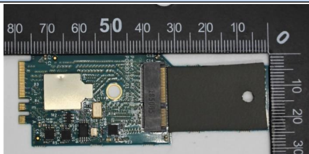
Extender board
