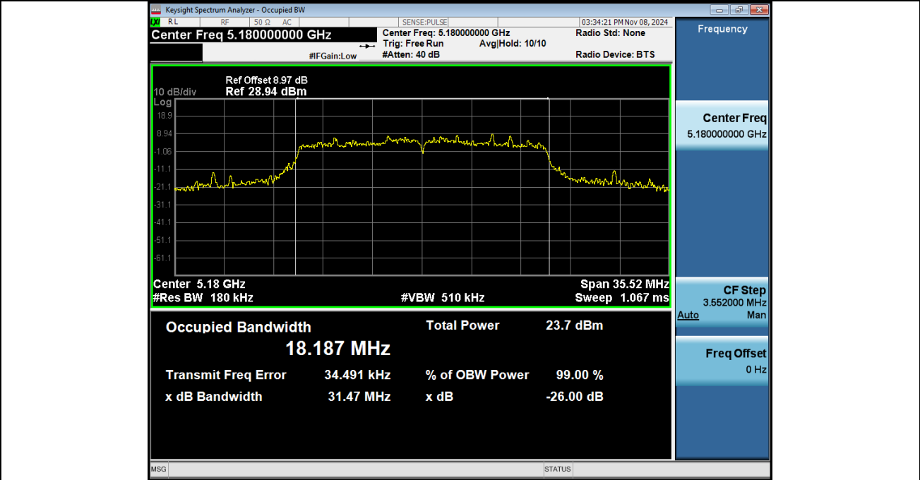
-26BW_NVNT_ANT2_802_11a_5180
