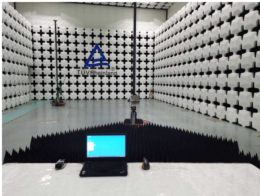
Photograph 3: Set-up photo for Radiated Emission, Above 1GHz
