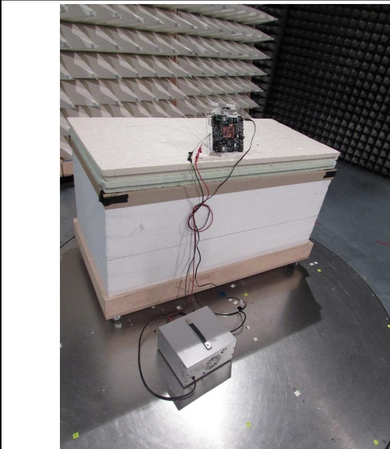
EUT Test Setup below 1 GH- Antenna 2
