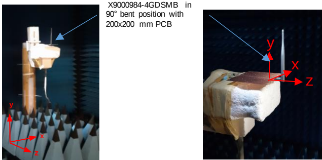
Antenna measured with PCB
