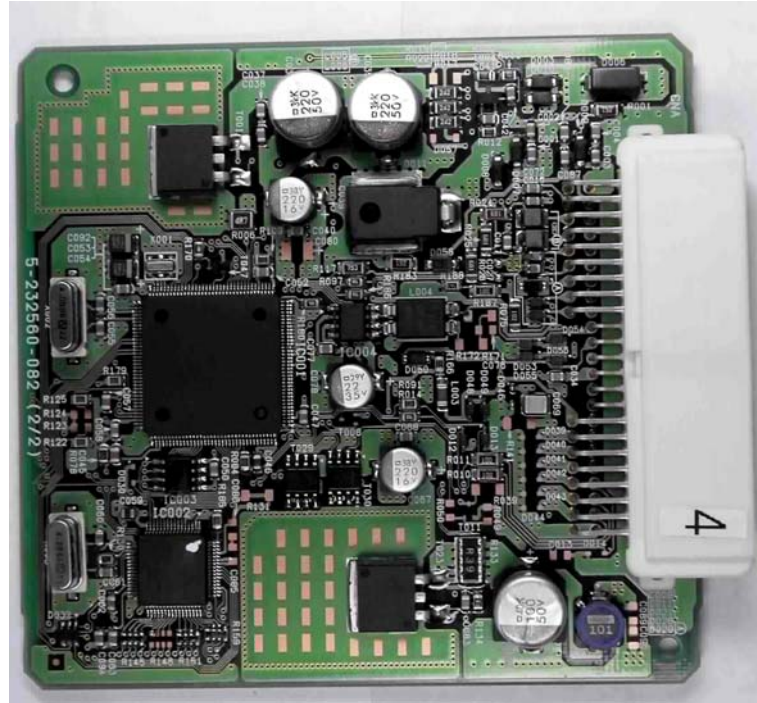
Computer Assy of TMLF-2 (PCB front view)
