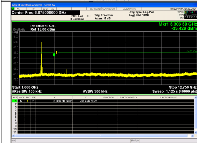
1000.0 MHz - 12750.0 MHz LE Channel 39
