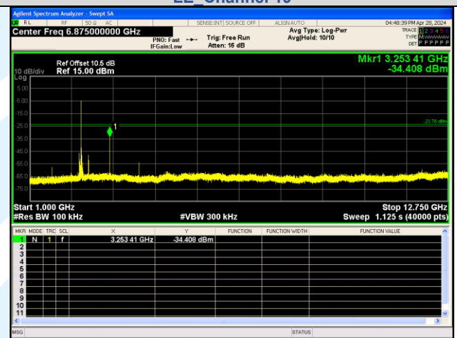
1000.0 MHz - 12750.0 MHz LE Channel 19
