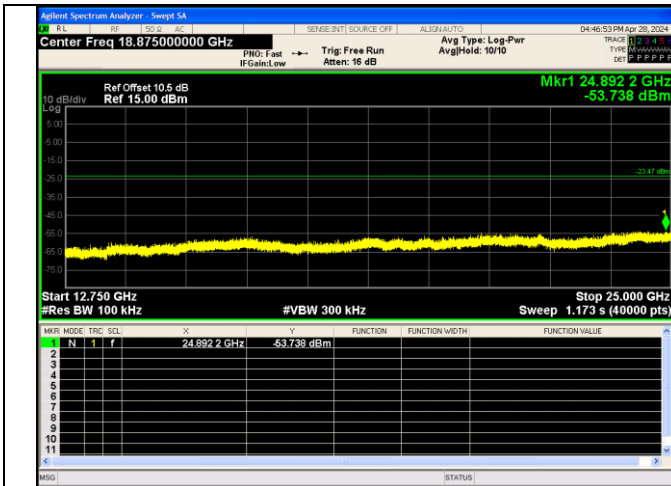
12750.0 MHz - 25000.0 MHz LE Channel 0
