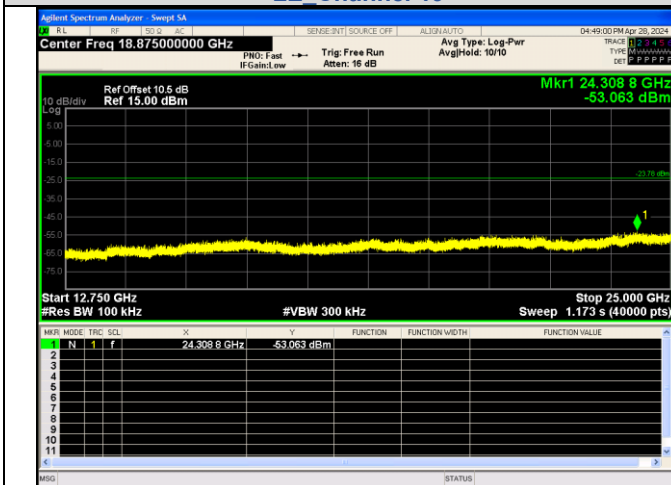
12750.0 MHz - 25000.0 MHz LE Channel 19
