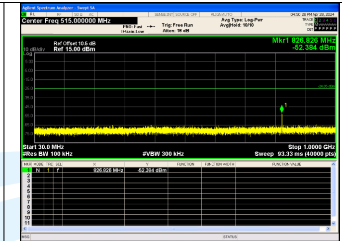
30.0 MHz - 1000.0 MHz LE Channel 39
