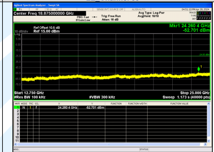
12750.0 MHz - 25000.0 MHz LE Channel 39
