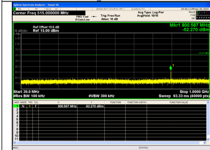
30.0 MHz - 1000.0 MHz LE Channel 0
