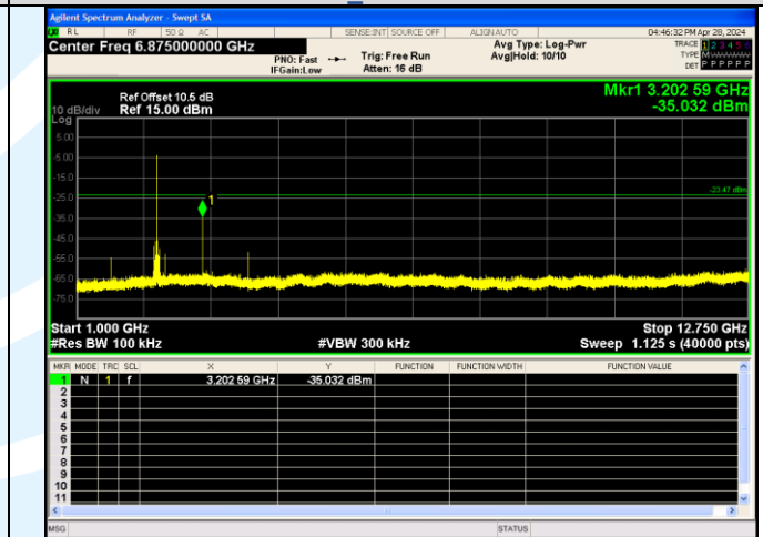
1000.0 MHz - 12750.0 MHz LE Channel 0
