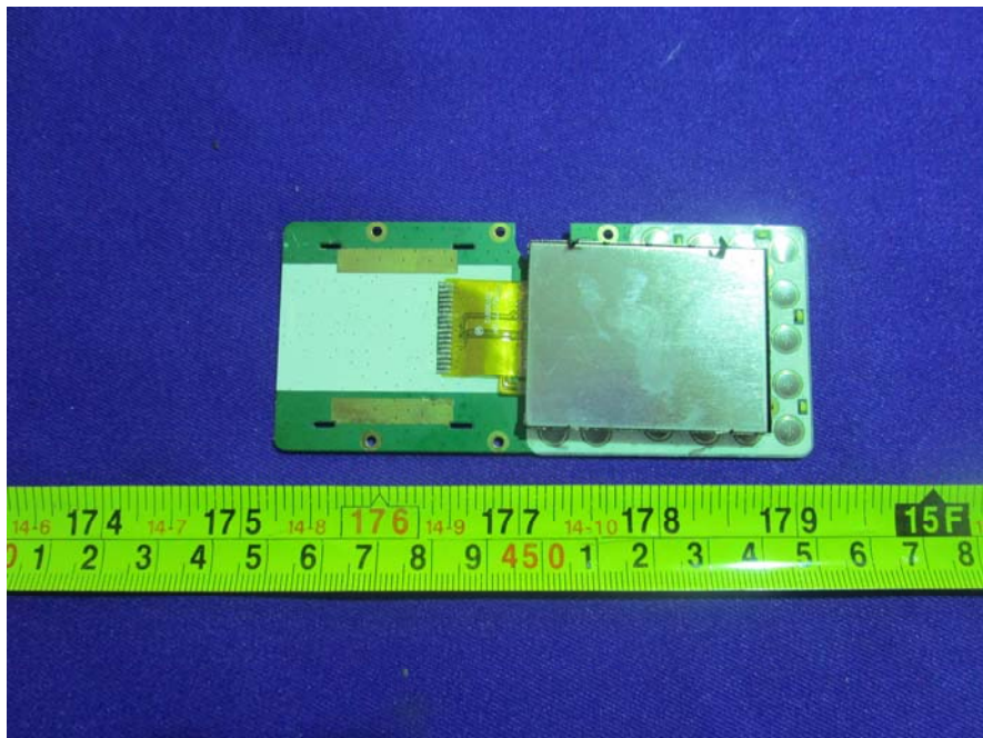
EUT –Subboard Top Uncover View
