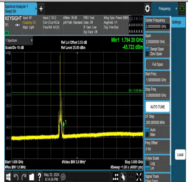
Band4_15MHz_QPSK_20325_1RB#0_1000~3000_1000~3000
