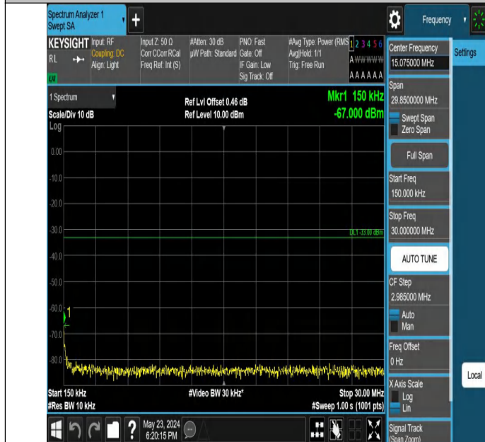
Band4_20MHz_QPSK_20175_1RB#99_0.15~30_0.15~30
