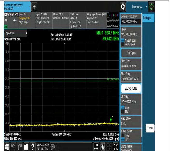
Band4_15MHz_QPSK_20325_1RB#74_30~1000_30~1000
