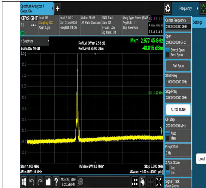
Band4_20MHz_QPSK_20175_1RB#99_1000~3000_1000~3000
