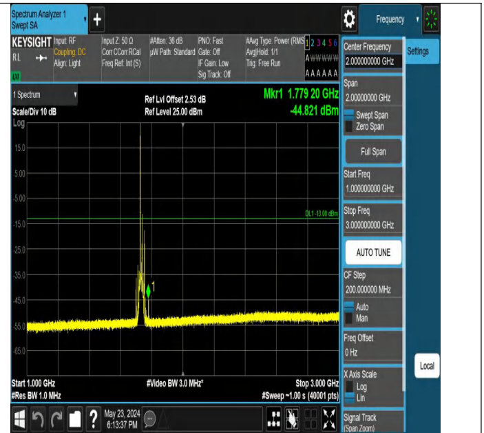
Band4_15MHz_QPSK_20175_1RB#0_1000~3000_1000~3000
