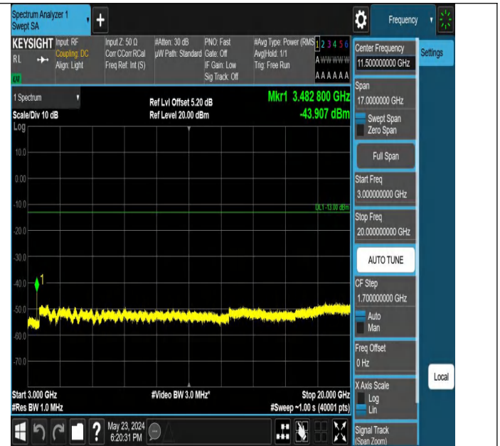
Band4_20MHz_QPSK_20175_1RB#99_3000~20000_3000~20000
