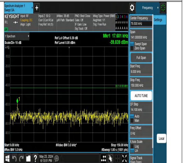
Band4_15MHz_QPSK_20175_1RB#74_0.009~0.15_0.009~0.15
