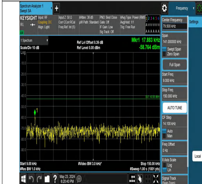
Band4_20MHz_QPSK_20300_1RB#0_0.009~0.15_0.009~0.15
