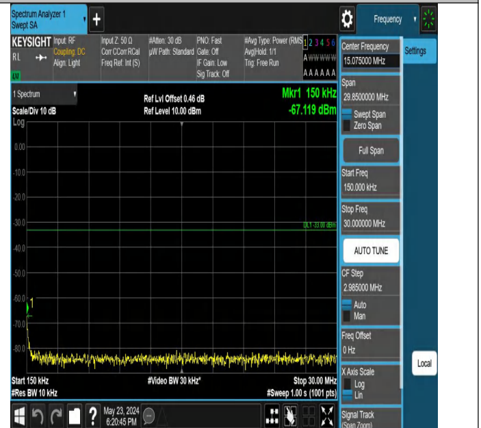
Band4_20MHz_QPSK_20300_1RB#0_0.15~30_0.15~30
