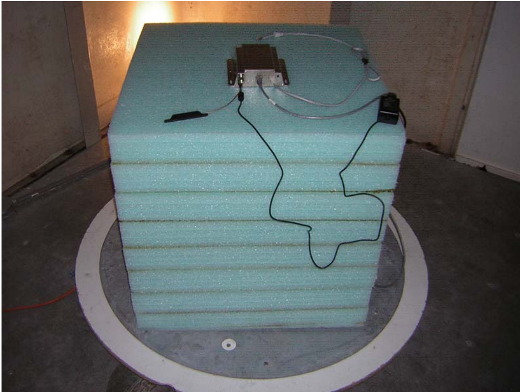
Radiated Emissions – Miltope antenna PN: 901167-1
