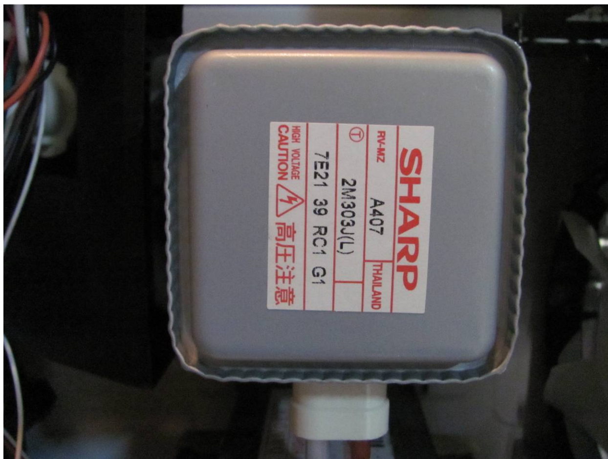
Figure 1. Magnetron
