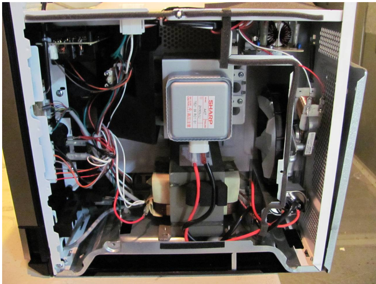
Figure 2. Magnetron Location
