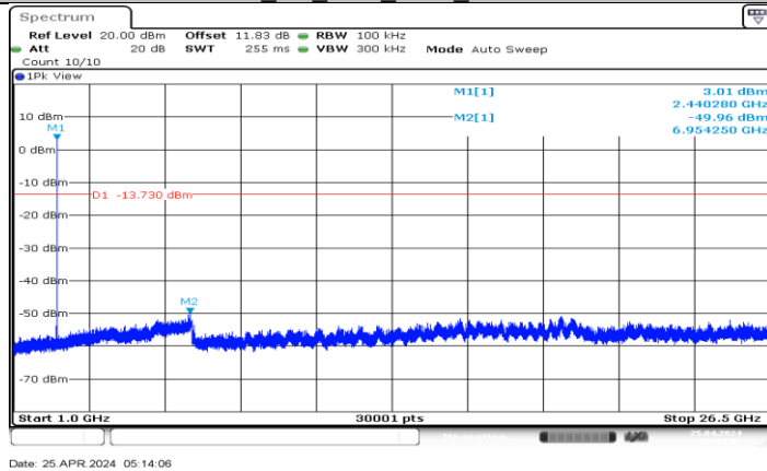
BLE_2M_Ant7_2440_1000~26500
