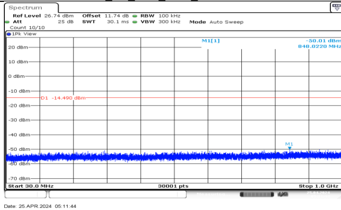
BLE_2M_Ant7_2402_30-1000
