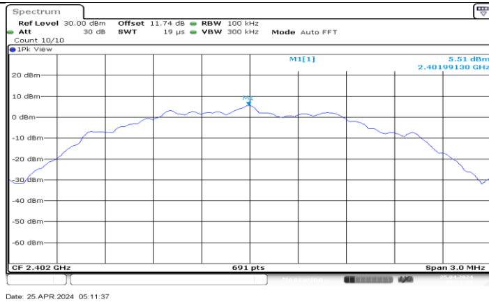
BLE_2M_Ant7_2402_0-Reference
