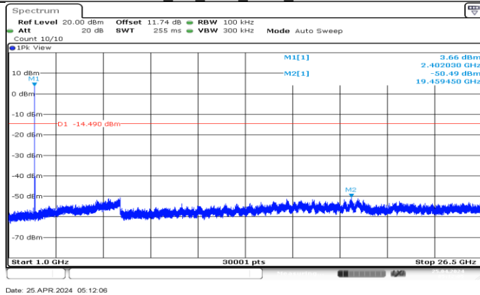
BLE_2M_Ant7_2402_1000-26500
