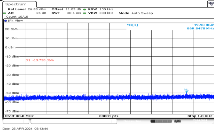
BLE_2M_Ant7_2440_30~1000
