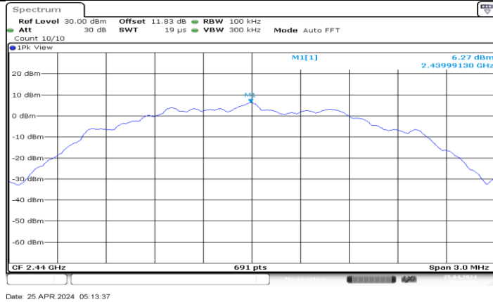
BLE_2M_Ant7_2440_0~Reference
