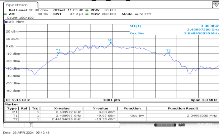
BLE_2M_Ant7_2440
