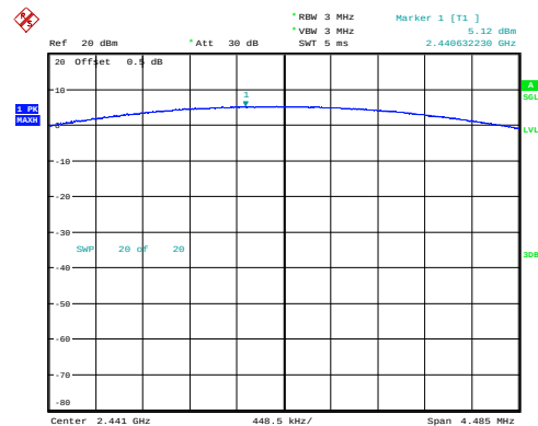
GFSK_Middle 5.12dBm
