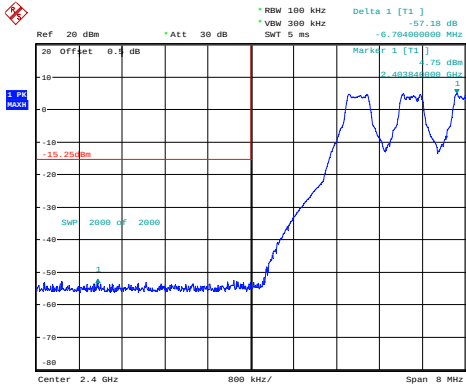
GFSK_Hopping_Lower 57.18dB
