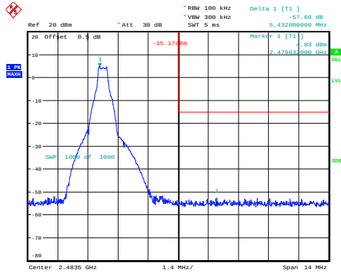
GFSK_High 57.69dB
