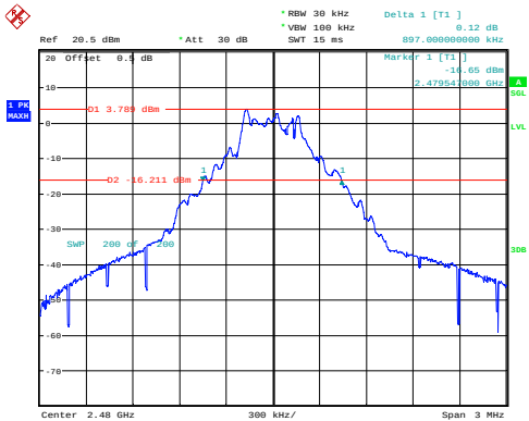
GFSK_High 0.897MHz
