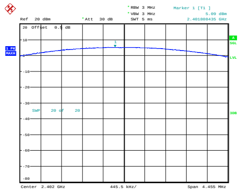
GFSK_Low 5.09dBm
