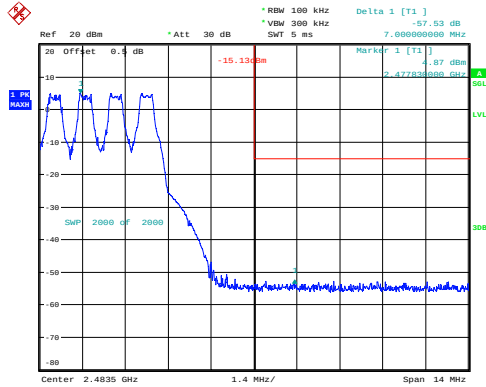
GFSK_Hopping_Upper 57.53dB
