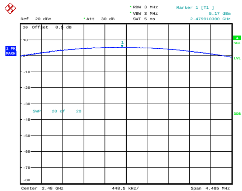
GFSK_High 5.17dBm
