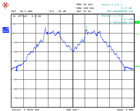
GFSK_Low 0.996MHz
