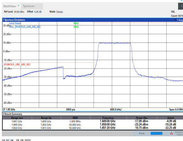
Band25-1.4MHz-QPSK-26047-6RB#0
