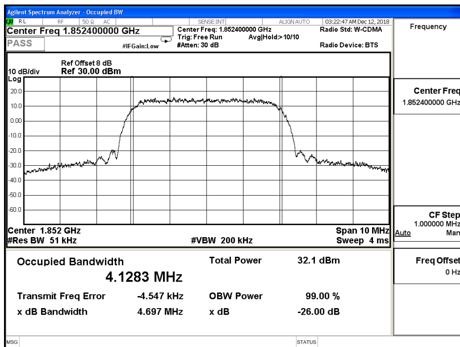
WCDMA_Band 2_RMC_1852.4MHz
