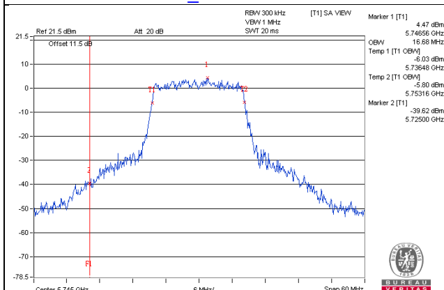
802.11ac (VHT20)_Chain0 / CH149
