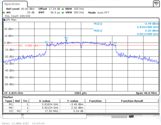
11N20MIMO-Ant1-5825-PASS
