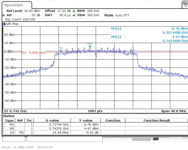
11N40MIMO-Ant2-5745-PASS
