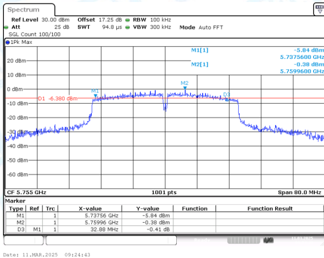
11AC40MIMO-Ant2-5755-PASS
