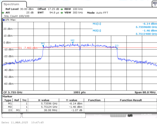
11AX40MIMO-Ant2-5755-PASS
