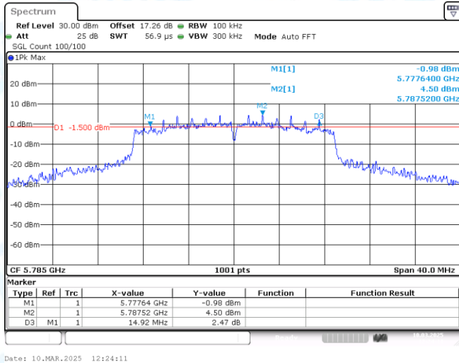
11N20MIMO-Ant2-5785-PASS
