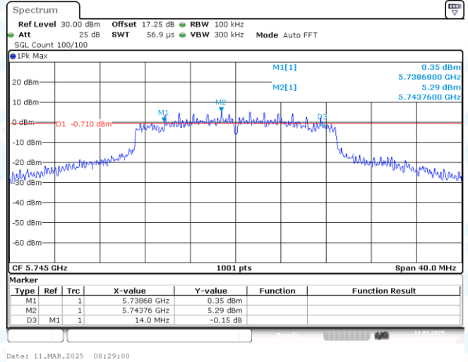
11AC20MIMO-Ant1-5745-PASS
