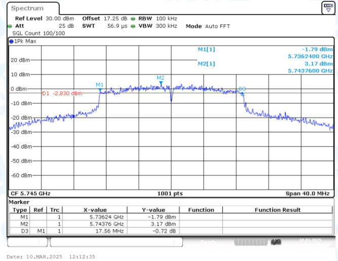
11N20MIMO-Ant1-5745-PASS
