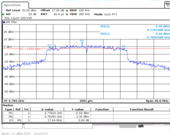
11AX20MIMO-Ant2-5785-PASS
