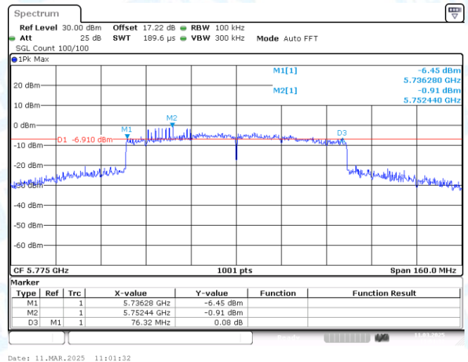
11AX80MIMO-Ant1-5775-PASS
