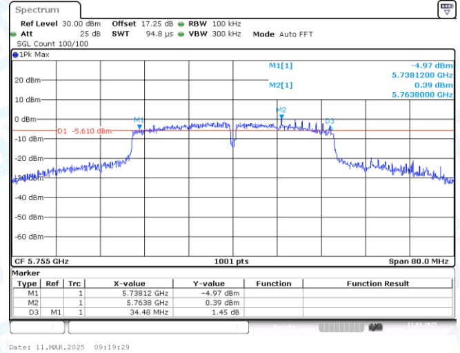
11AC40MIMO-Ant1-5755-PASS
