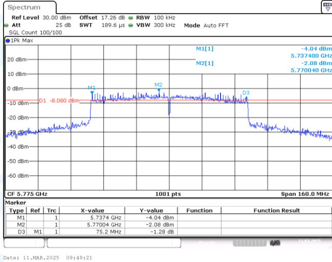
11AC80MIMO-Ant2-5775-PASS
