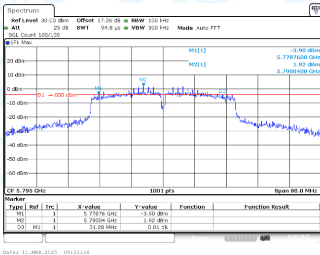
11AC40MIMO-Ant2-5795-PASS
