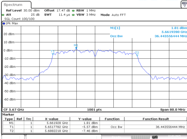
11AX40MIMO-Ant2-5670
