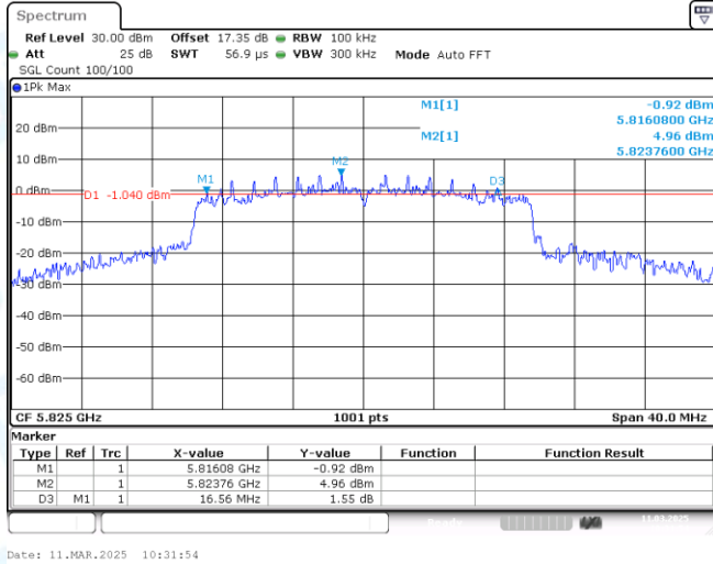
11AX20MIMO-Ant2-5825-PASS
