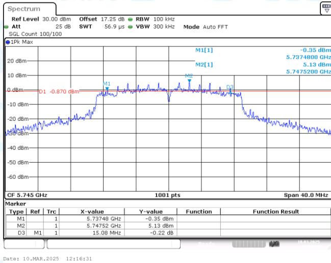
11N20MIMO-Ant2-5745-PASS
