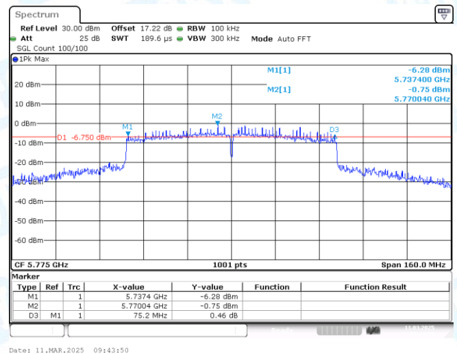
11AC80MIMO-Ant1-5775-PASS
