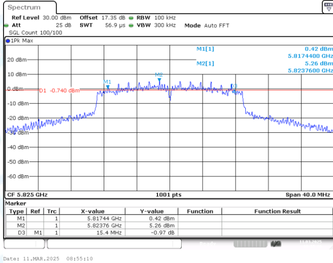
11AC20MIMO-Ant2-5825-PASS
