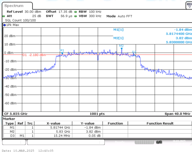
11N20MIMO-Ant2-5825-PASS
