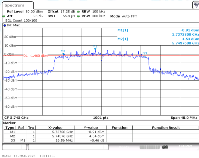
11AX20MIMO-Ant2-5745-PASS
