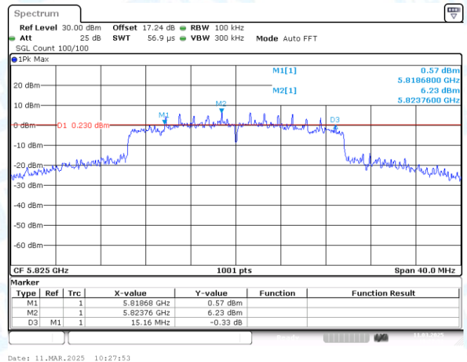
11AX20MIMO-Ant1-5825-PASS
