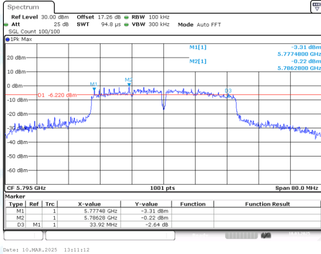
11N40MIMO-Ant2-5795-PASS
