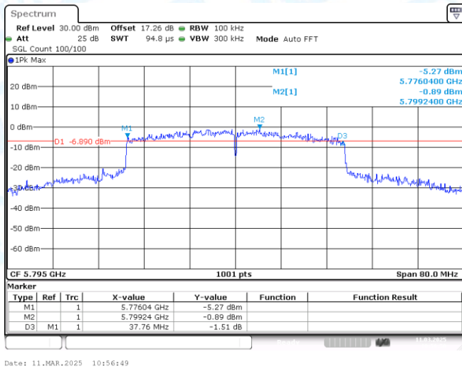
11AX40MIMO-Ant2-5795-PASS
