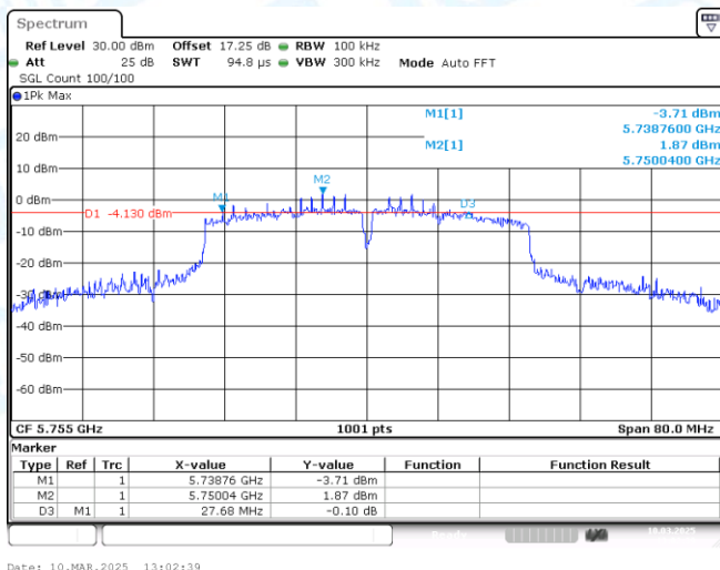
11N40MIMO-Ant2-5755-PASS
