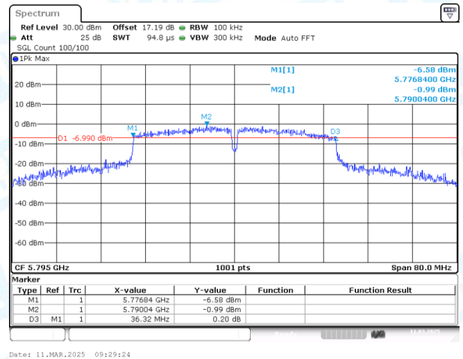
11AC40MIMO-Ant1-5795-PASS
