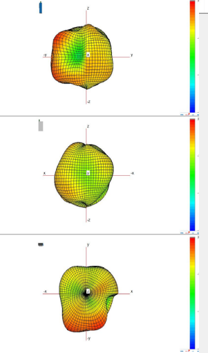
2484MHz 3D Antenna Pattern
