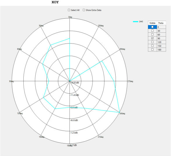
2D Antenna Pattern (X->Y;X->Z;Y->Z)
