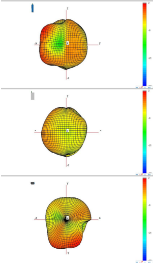
2484MHz 3D Antenna Pattern
