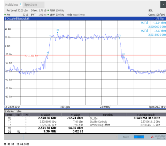
1-N38--30-10-L-2-DFT-PI2BPSK-Outer_Full-24@0-Ant0 -8.544-9.360-≤10-PASS
