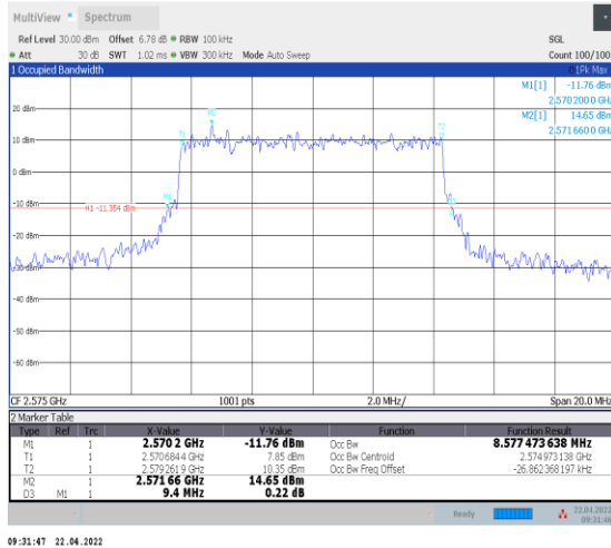
1-N38--30-10-L-1-DFT-QPSK-Outer_Full-24@0-Ant0 -8.577-9.400-≤10-PASS
