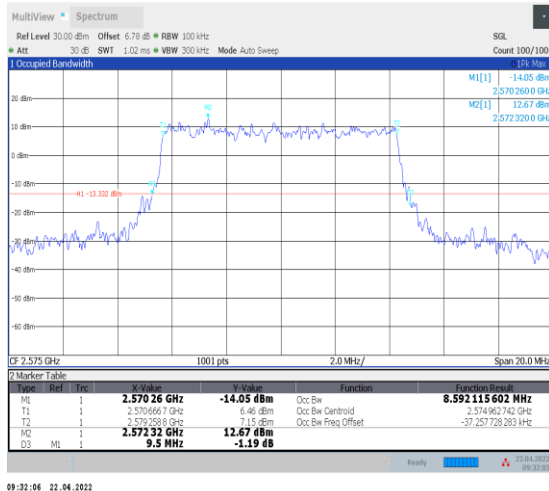
1-N38--30-10-L-3-DFT-16QAM-Outer_Full-24@0-Ant0 0-8.592-9.500-≤10-PASS
