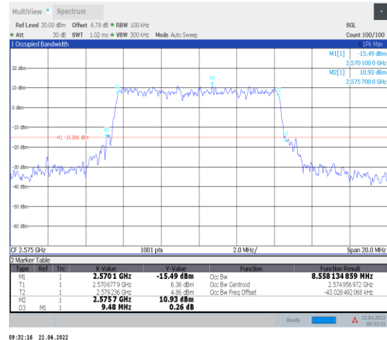
1-N38--30-10-L-4-DFT-64QAM-Outer_Full-24@0-Ant0 t0-8.558-9.480-≤10-PASS
