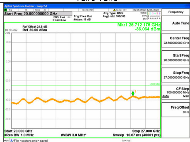
41C-20G-27G / 15+20MHz / QPSK / High CH / 1#0-1#99
