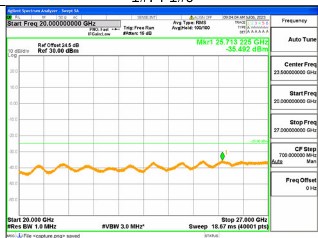
41C-20G-27G / 15+15MHz / QPSK / High CH / 75#0-75#0
