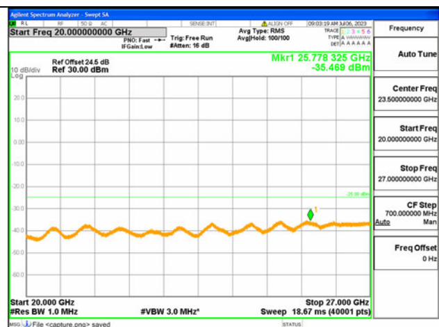
41C-20G-27G / 15+15MHz / QPSK / High CH / 1#74-1#0
