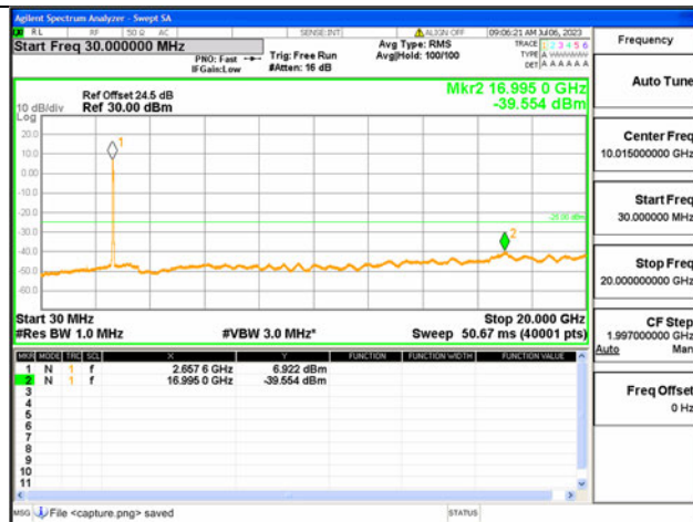
41C-30M-20G / 15+20MHz / QPSK / High CH / 75#0-100#0
