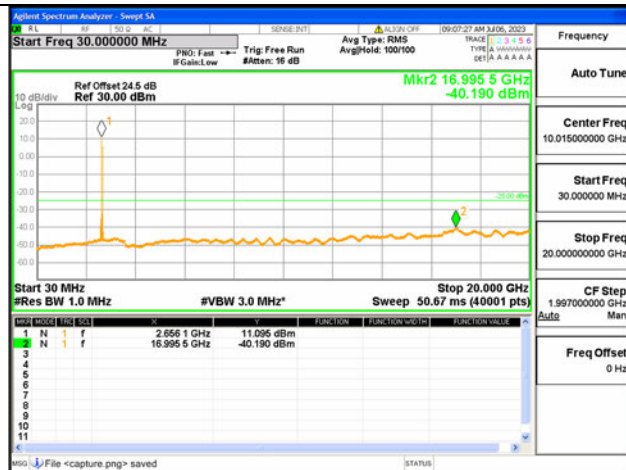
41C-30M-20G / 20+15MHz / QPSK / High CH / 1#0-1#74
