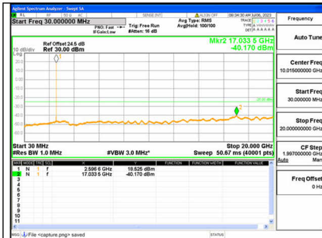
41C-30M-20G / 20+10MHz / QPSK / Mid CH / 1#99-1#0
