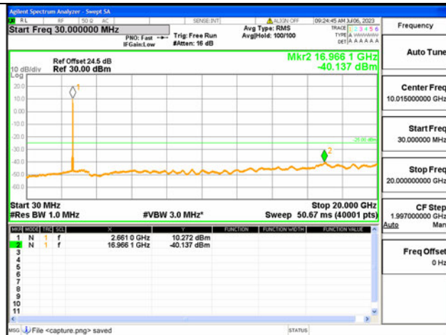
41C-30M-20G / 20+10MHz / QPSK / High CH / 1#0-1#49
