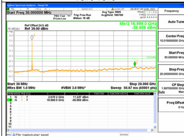
41C-30M-20G / 15+20MHz / QPSK / Mid CH / 1#0-1#99
