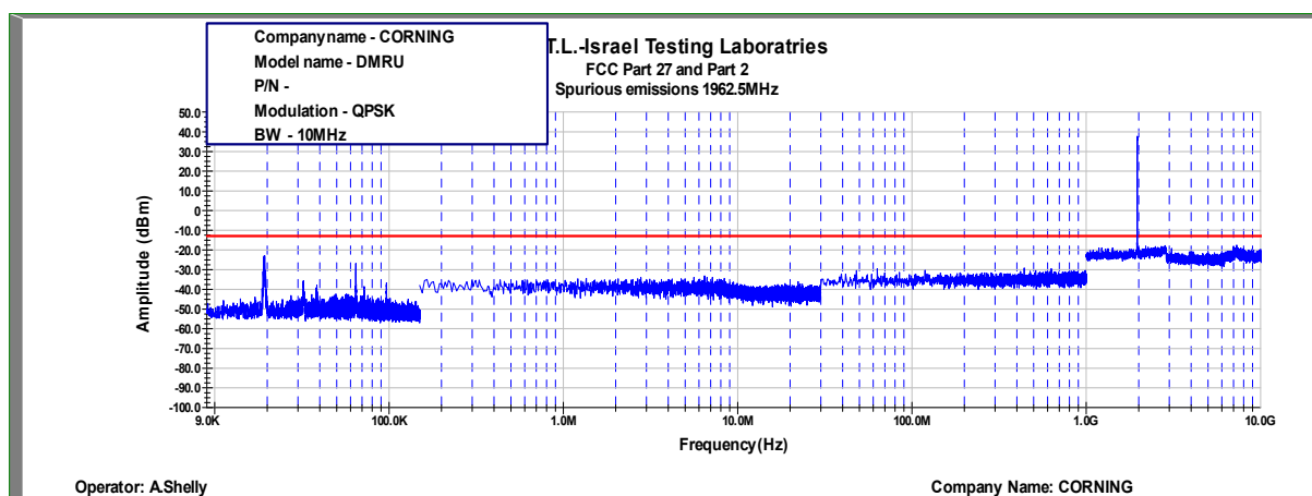
Figure 480: Spurious Emissions at Antenna Terminal QPSK, 1962.5MHz, B.W. 10MHz – 4G
