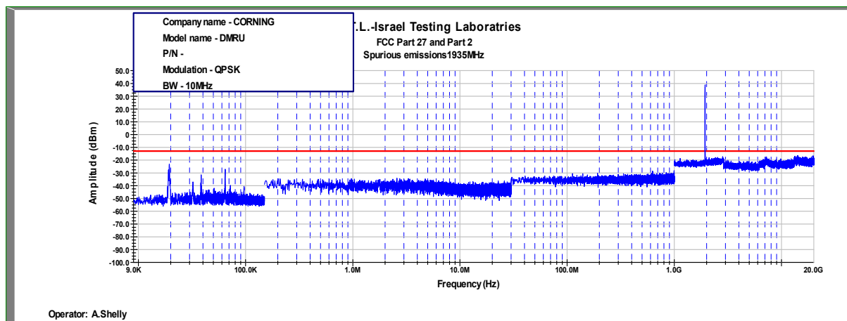
Figure 479: Spurious Emissions at Antenna Terminal QPSK, 1935MHz, B.W. 10MHz – 4G
