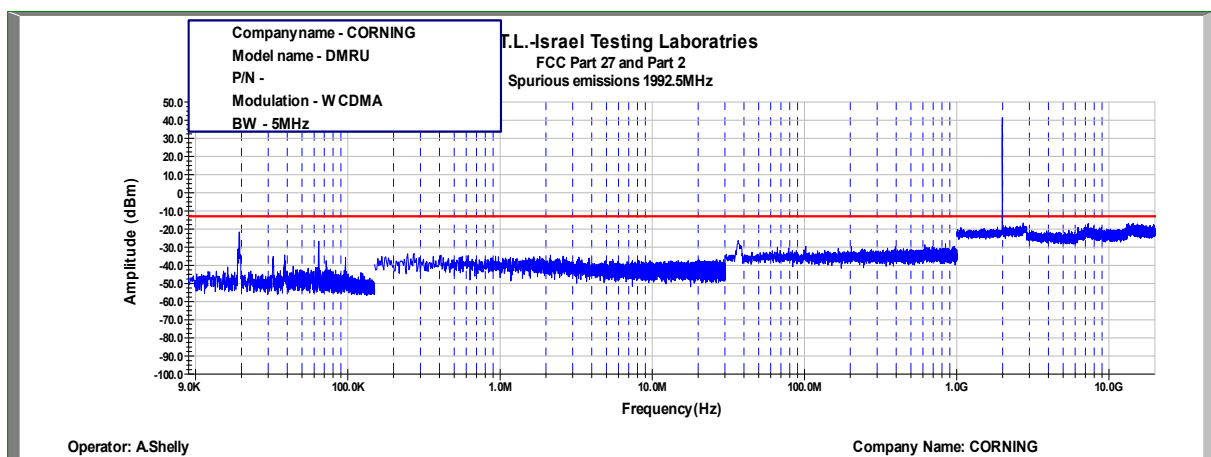
Figure 457: Spurious Emissions at Antenna Terminal WCDMA, 1992.5MHz, B.W. 5MHz- 3G
