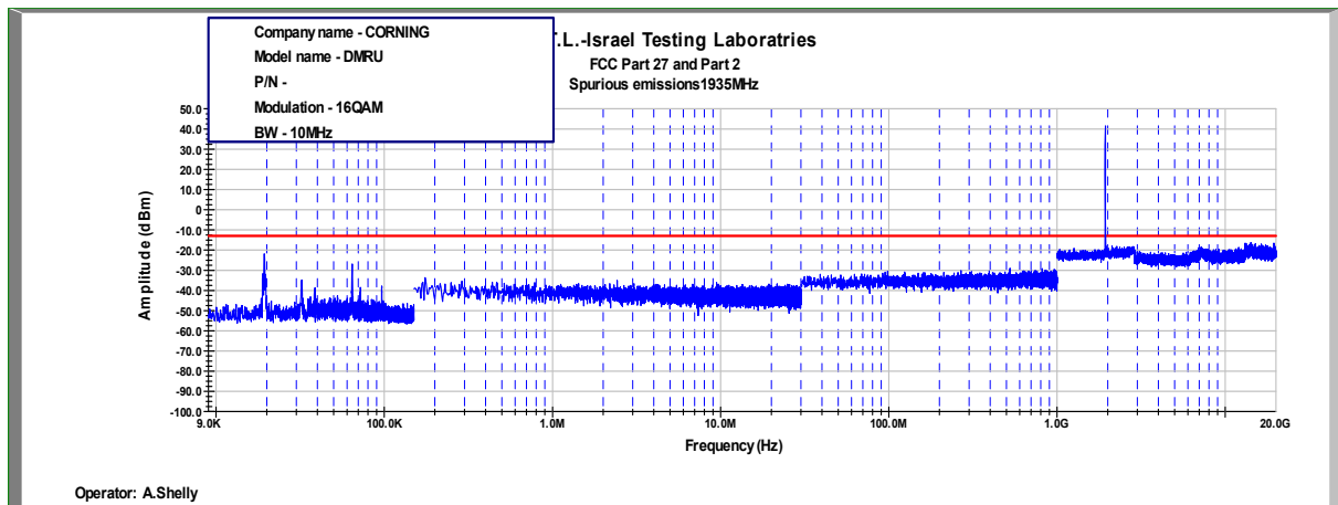
Figure 461: Spurious Emissions at Antenna Terminal 16QAM, 1935MHz, B.W. 10MHz – 4G
