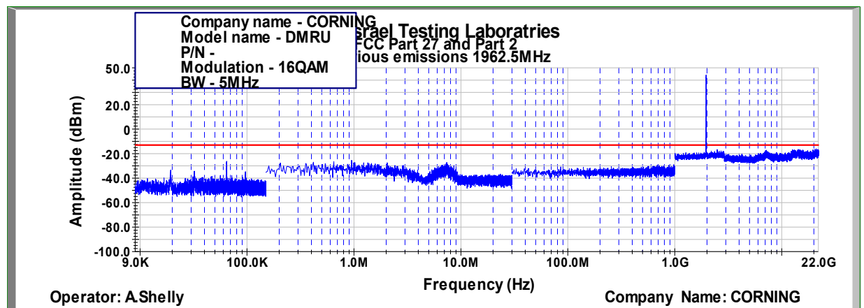
Figure 459: Spurious Emissions at Antenna Terminal 16QAM, 1962.5MHz, B.W. 5MHz
